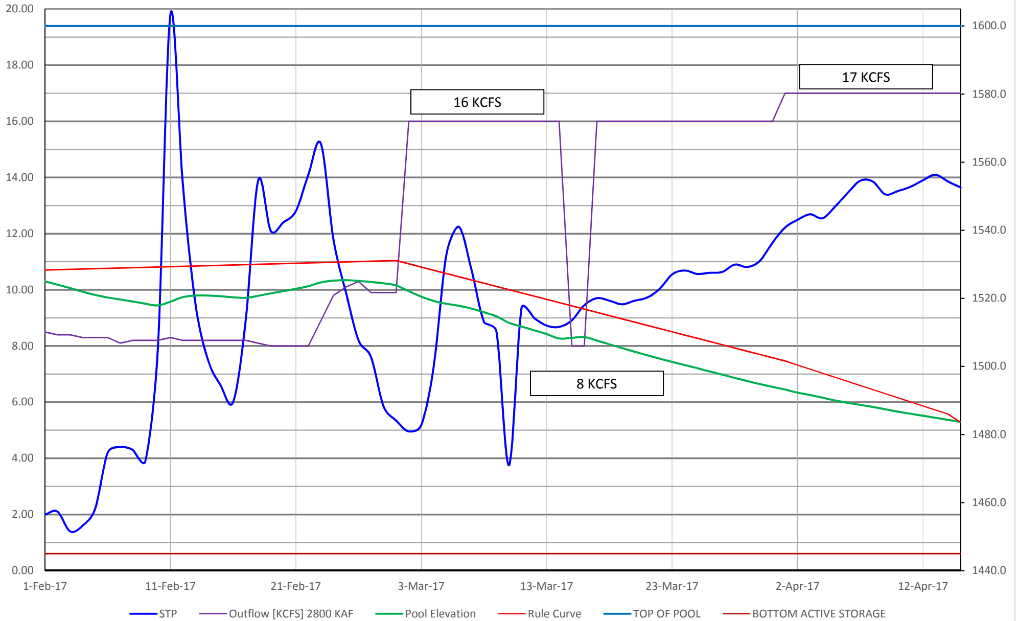
STP + Fish Release Dworshak Inflows 2.8 MAF 15 Apr Operation
