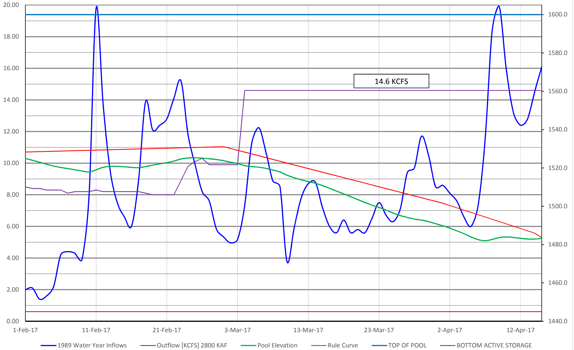
1989 Dworshak Inflows 2.8 MAF 15 Apr Operation
