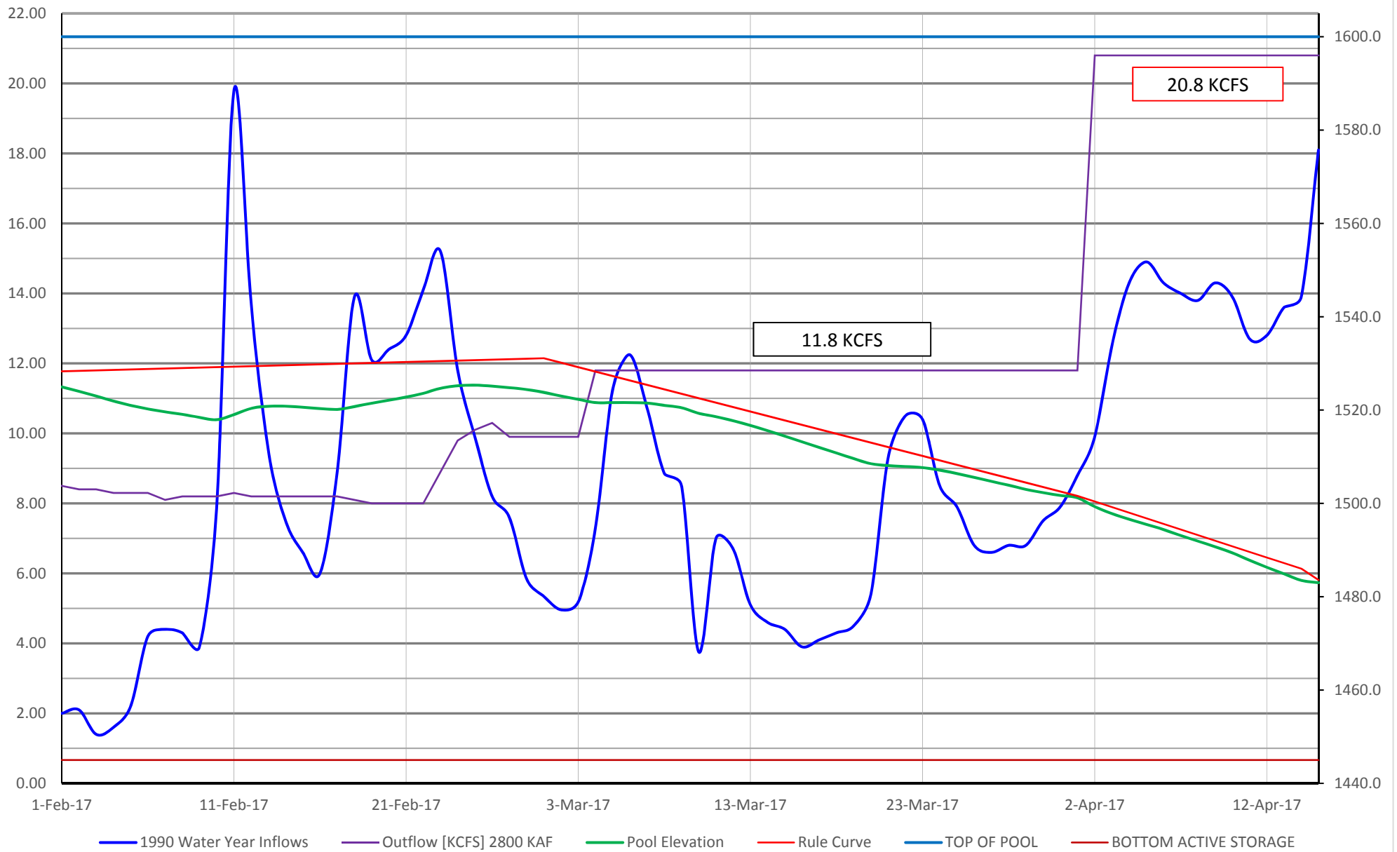
1990 Dworshak Inflows 2.8 MAF Typ Flood Risk Management
