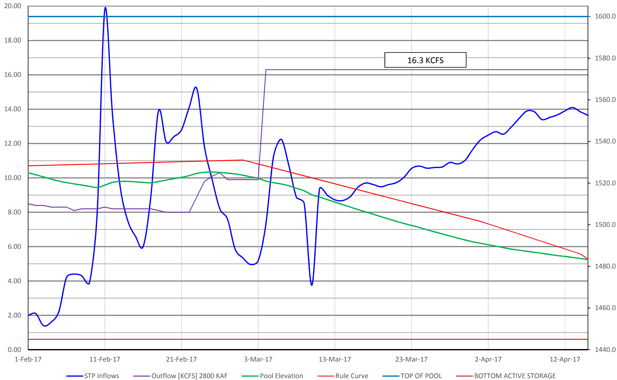
STP Dworshak Inflows 2.8 MAF 15 Apr Operation
