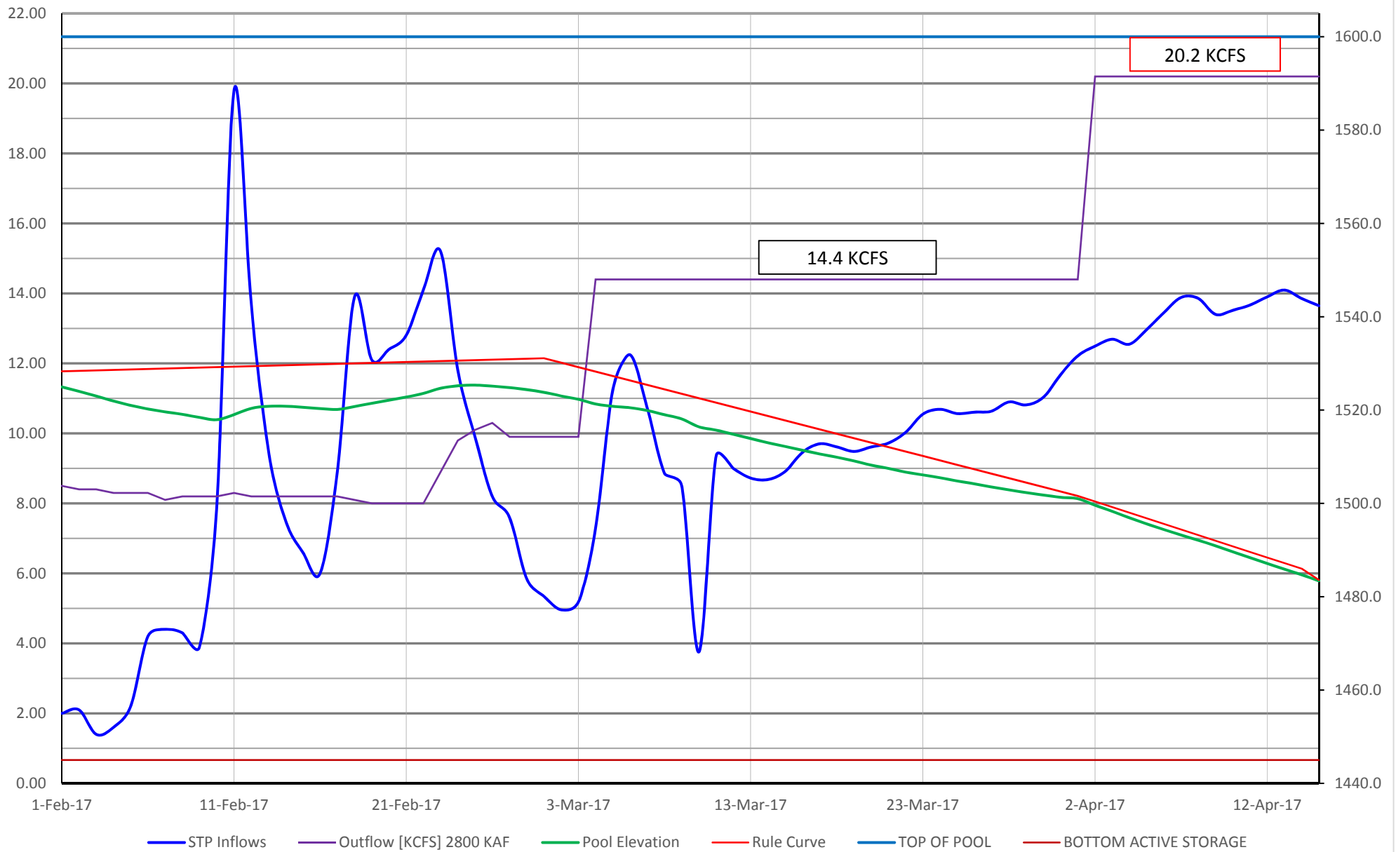
STP Dworshak Inflows 2.8 MAF Typ Flood Risk Management
