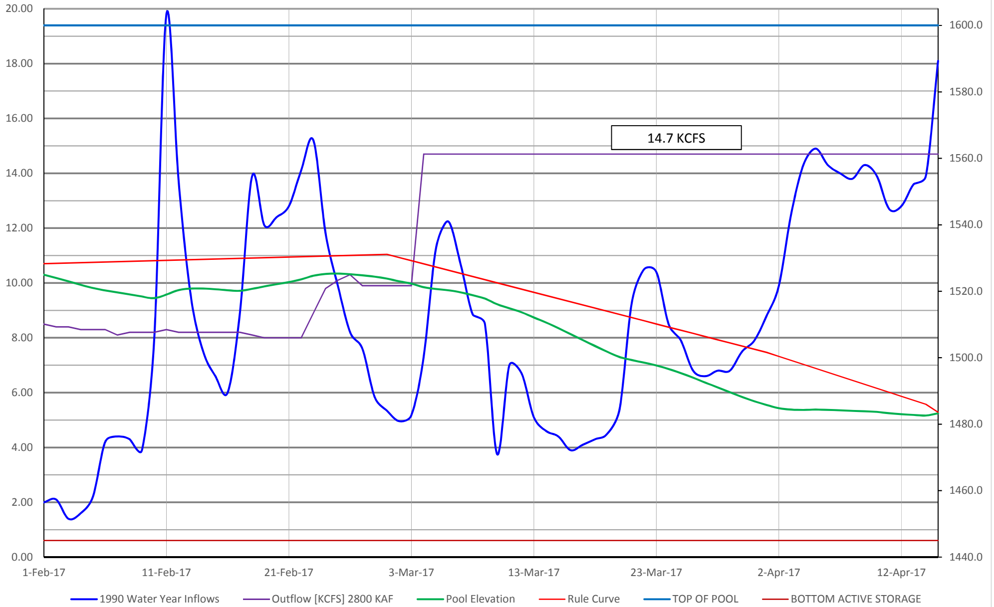
1990 Dworshak Inflows 2.8 MAF 15 Apr Operation
