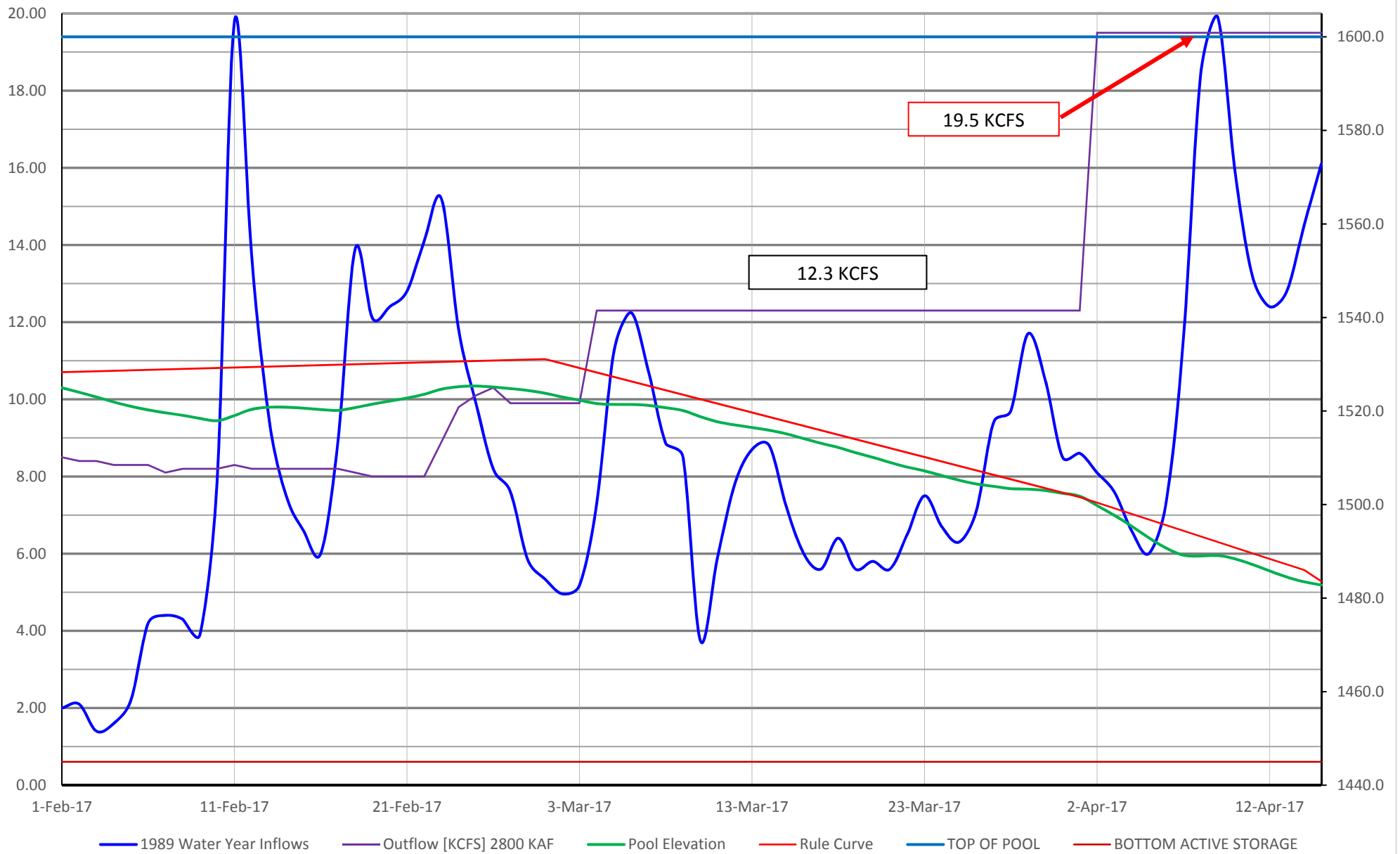
1989 Dworshak Inflows 2.8 MAF Typ Flood Risk Management
