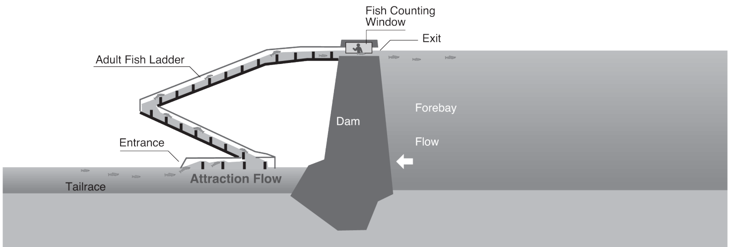
Figure OV-1 Generalized Example of Types of Fish Passage Structures at a Dam OV-12
