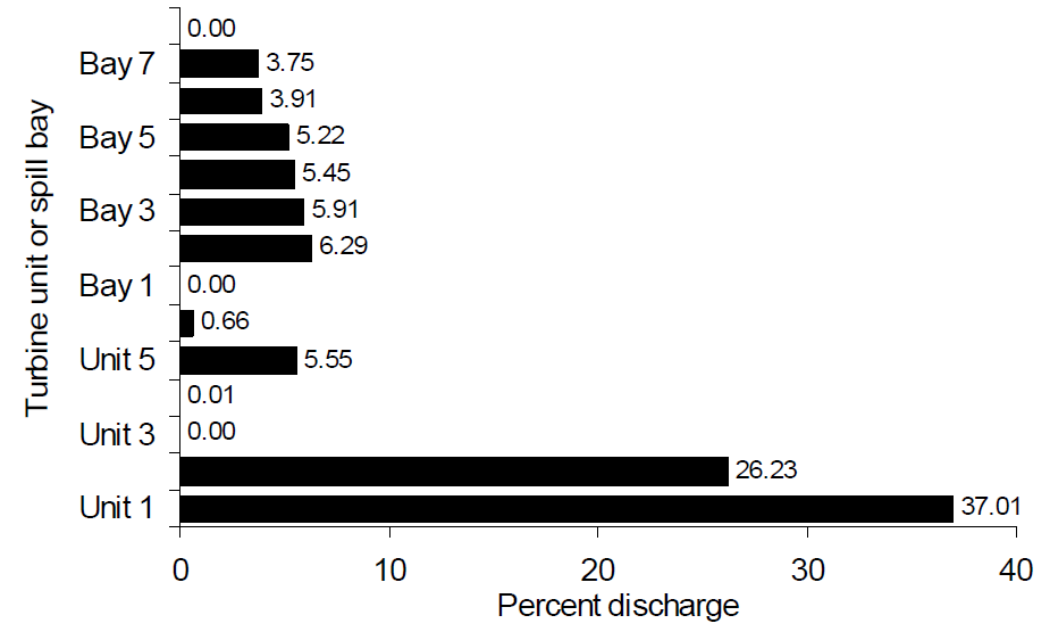
Figure 34. — Percent of total discharge through each turbine unit or spill bay during the Uniform spill pattern at Little Goose Dam, summer 2007.
