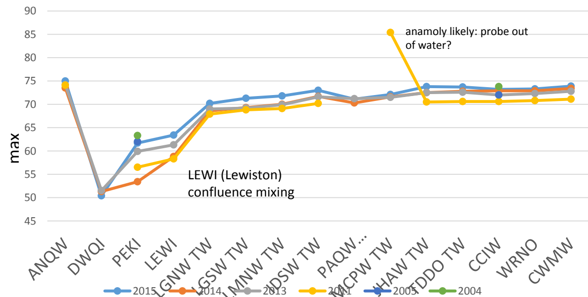
Columbia basin water temperature: maximum degF in Tailwater stations (probes ~15 feet deep)
