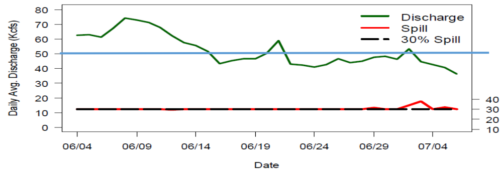
Figure 3.1. Daily average total discharge (kcfs) (green line) and percent spill (red line) at Little Goose Dam during the summer subyearling Chinook salmon study, 4 June to 6 July 2013. The black dashed line represents 30% spill.
