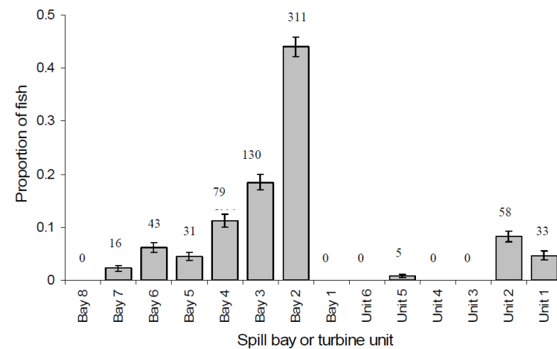
Figure 44. — Proportion of subyearling Chinook salmon passing through each spill bay or turbine unit at Little Goose Dam, summer 2007. Whisker bars represent the standard error of a proportion and numbers above bars are sample sizes.
