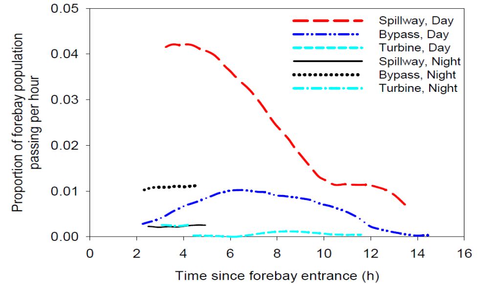
Figure 43. — Rates of dam passage of subyearling Chinook salmon entering the Little Goose Dam forebay during the day (approximately 0430- 2115) and night during 2007.
