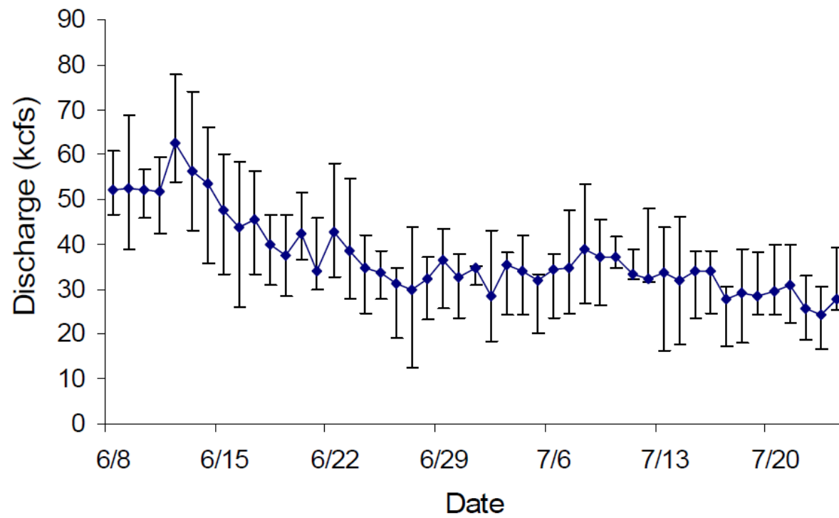
Figure 33. — Mean daily discharge through Little Goose Dam, summer 2007. Whisker bars represent the daily minimum and maximum discharge.
