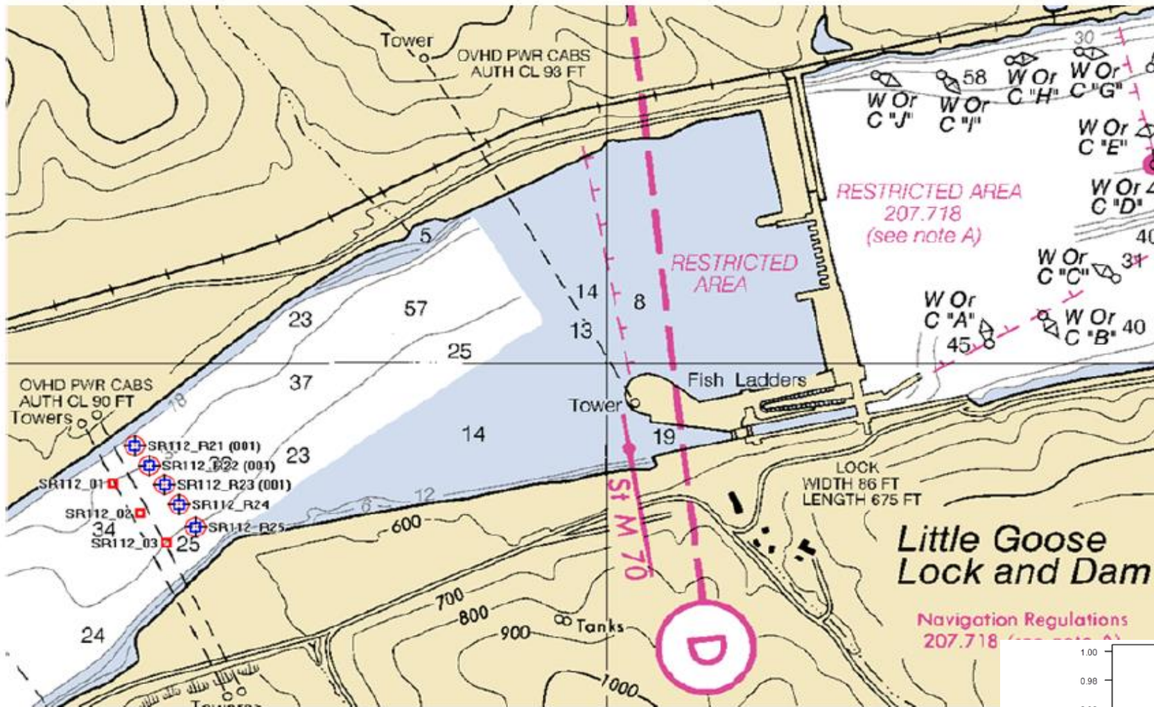
Figure 3.6. Little Goose Dam tailrace fish release locations (red circle with blue sq position 1 (SR112_R21) is near the north shore and release position nu (SR112_R25) is near the south shore.
