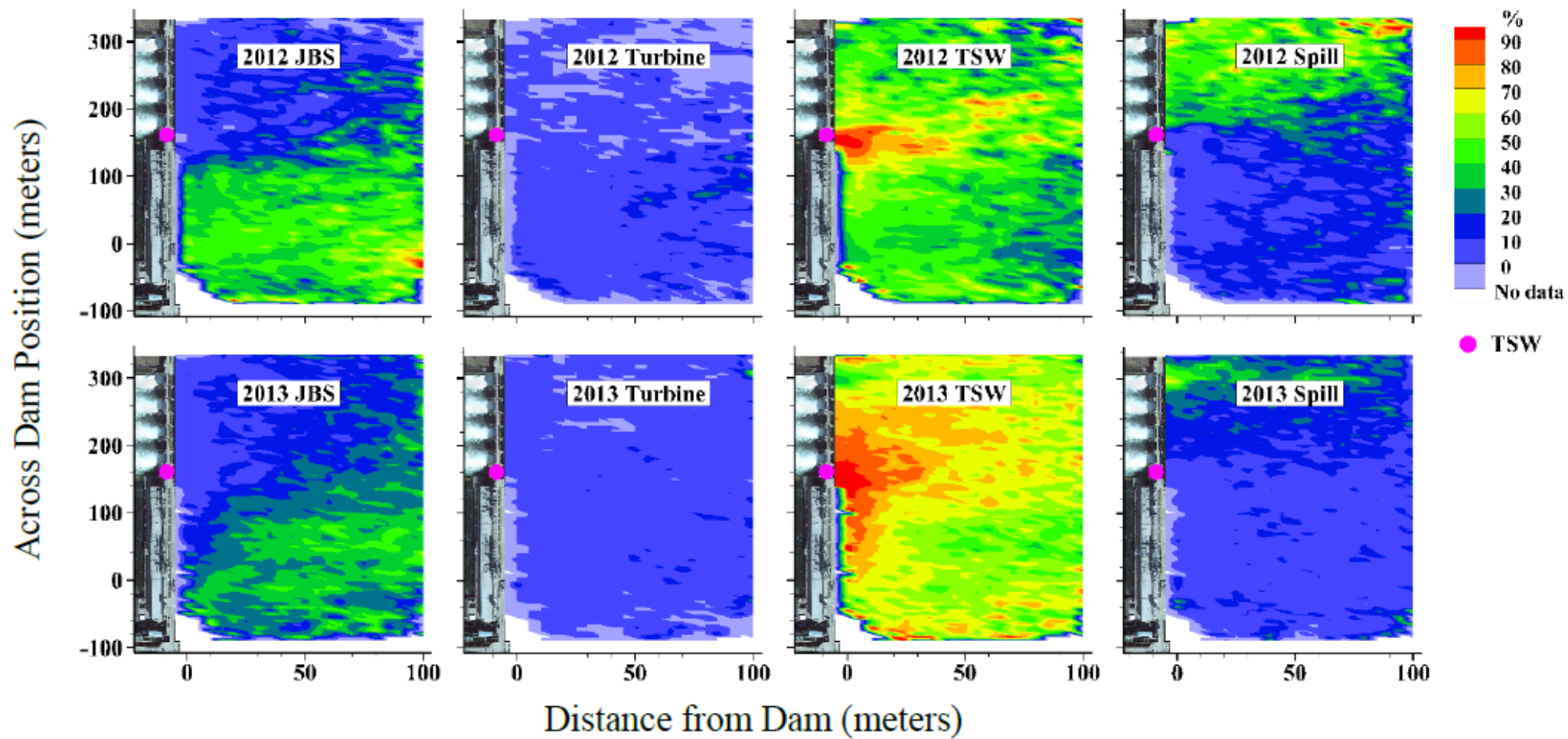
Figure 3.2. Passage probabilities by forebay location and route for acoustic-tagged subyearling Chinook salmon detected at depths between 7.5 m and 12.5 m from the water surface at Little Goose Dam in 2012 (top) and 2013 (bottom). The aerial photo incorporated on the left side of each plot illustrates the location of the spillway near the top of the axis and the powerhouse at the bottom of the axis. The temporary spillway weir is located at the first spill bay nearest the powerhouse and is marked with a pink dot overlaid onto the aerial photo.
