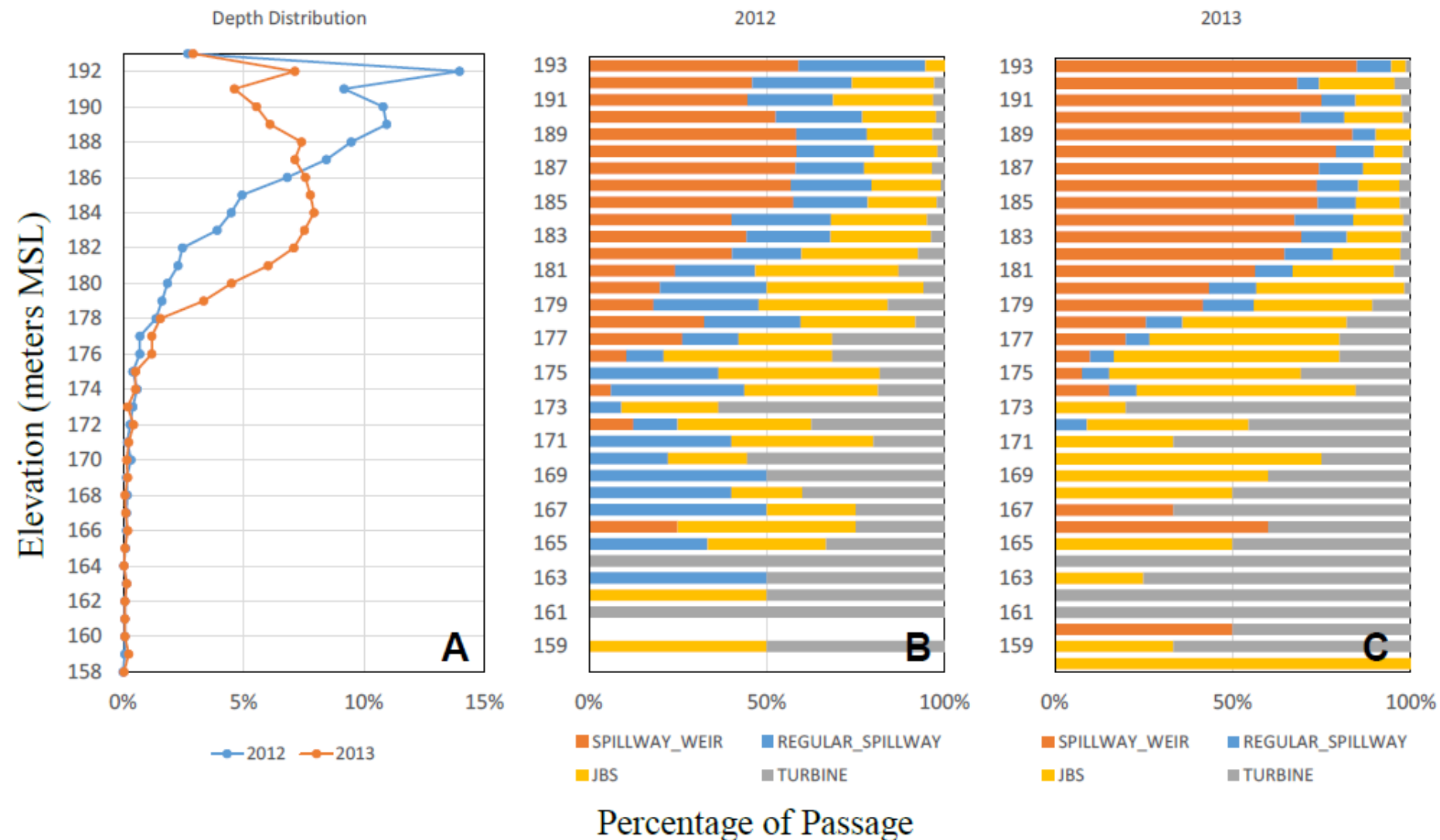
Figure 3.1. Vertical distributions of acoustic-tagged subyearling Chinook salmon that passed Little Goose Dam in 2012 and 2013 (A), 2012 routes of passage (B), and 2013 routes of passage (C).
