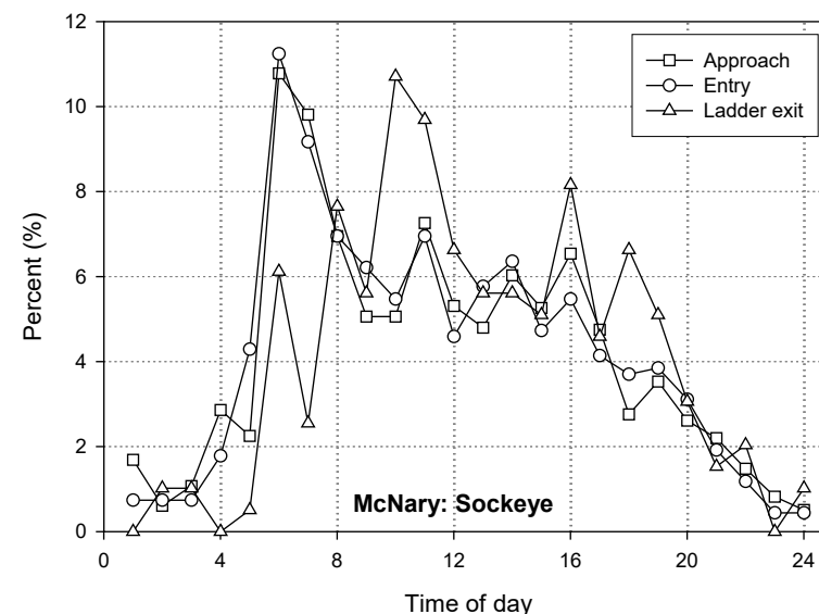
Figure MCN-2. Diel Distribution of Adult Salmonids at McNary Dam Fishway Entrances and Exits (Keefe & Caudill 2008). Report and summary letter available online at: https://public.crohms.org/tmt/documents/FPOM/2010/2013_FPOM_MEET/2013_JUN/
