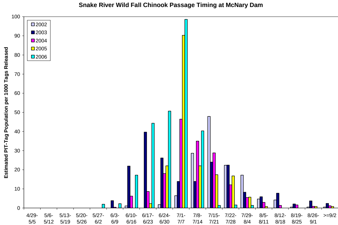
Passage timing of Snake River wild fall Chinook passing MCN (MY 2002-2006).
