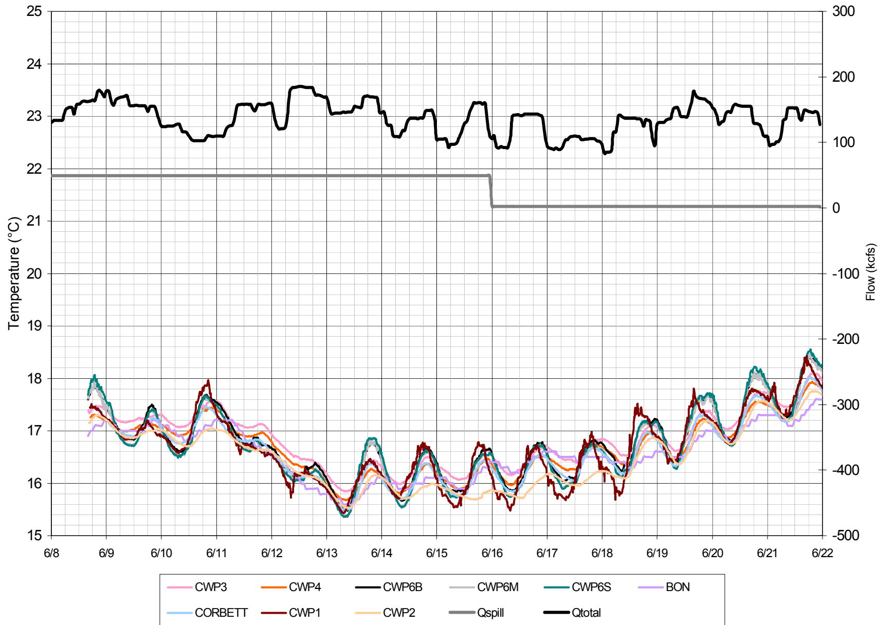
Figure 35. Hourly Columbia River water temperatures at river mile 122, June 2001. (lateral transect CWP1-CWP6 oriented Oregon to Washington shore)
