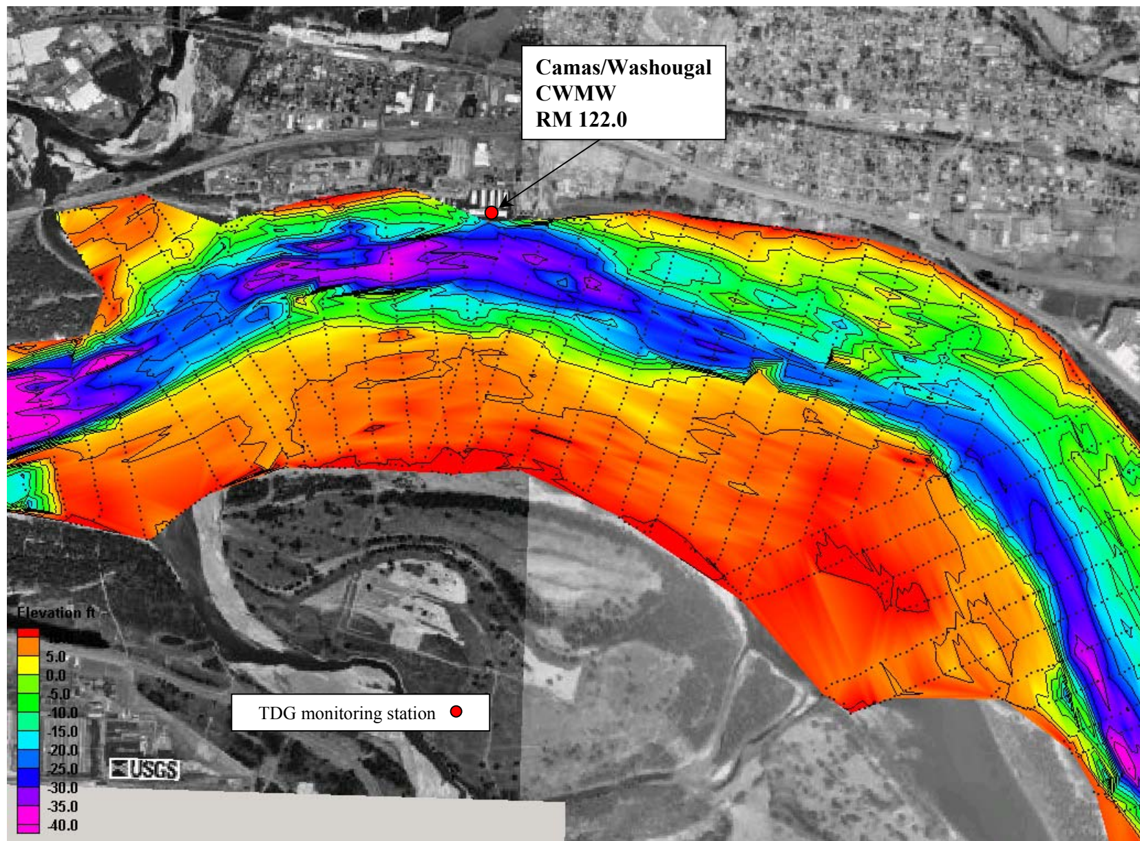
Figure 4. Columbia River Channel Elevations and TDG Fixed Monitoring Station near Camas/Washougal Washington.
