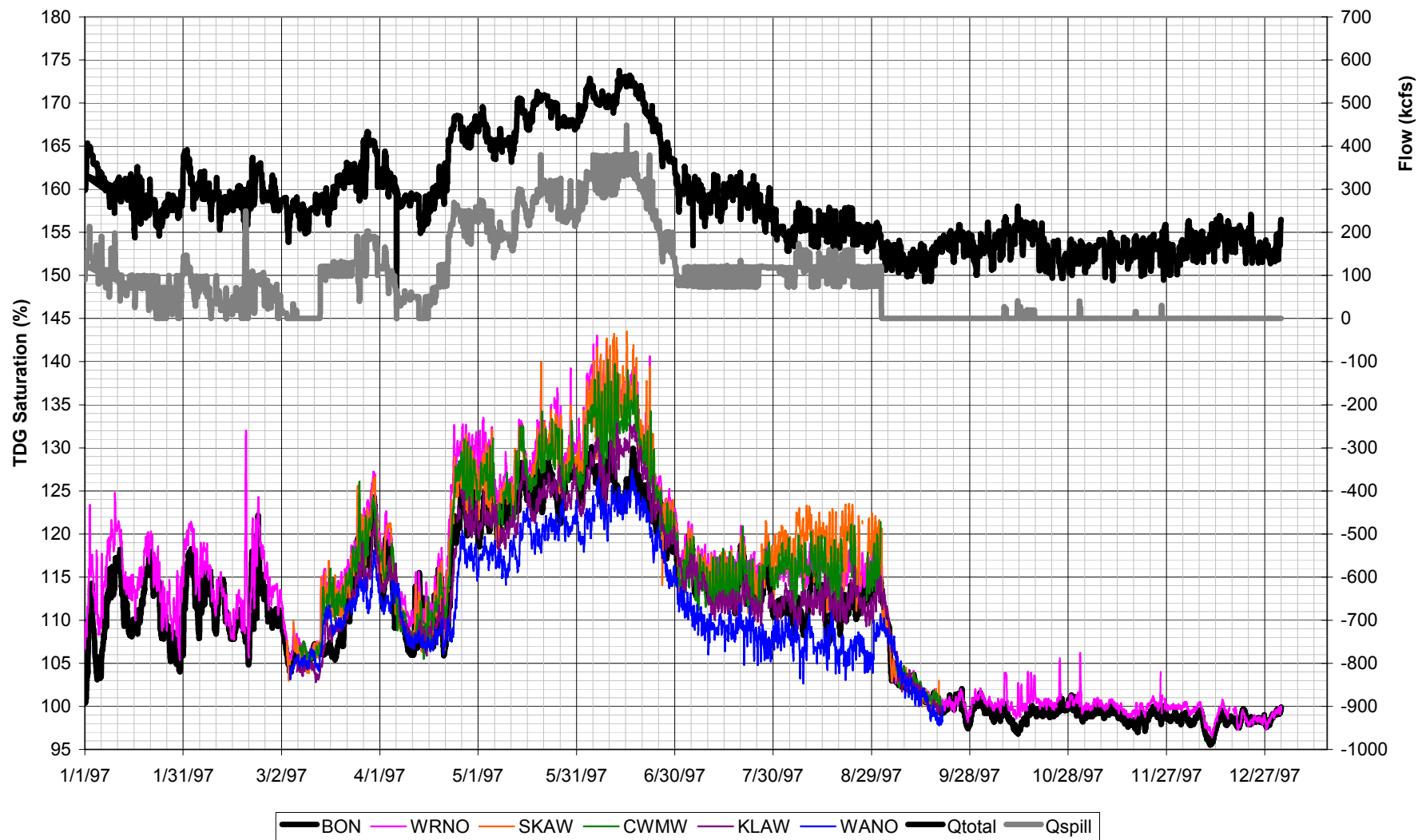
Figure 14. Bonneville Dam Flow and Columbia River Total Dissolved Gas Saturation, 1997.
