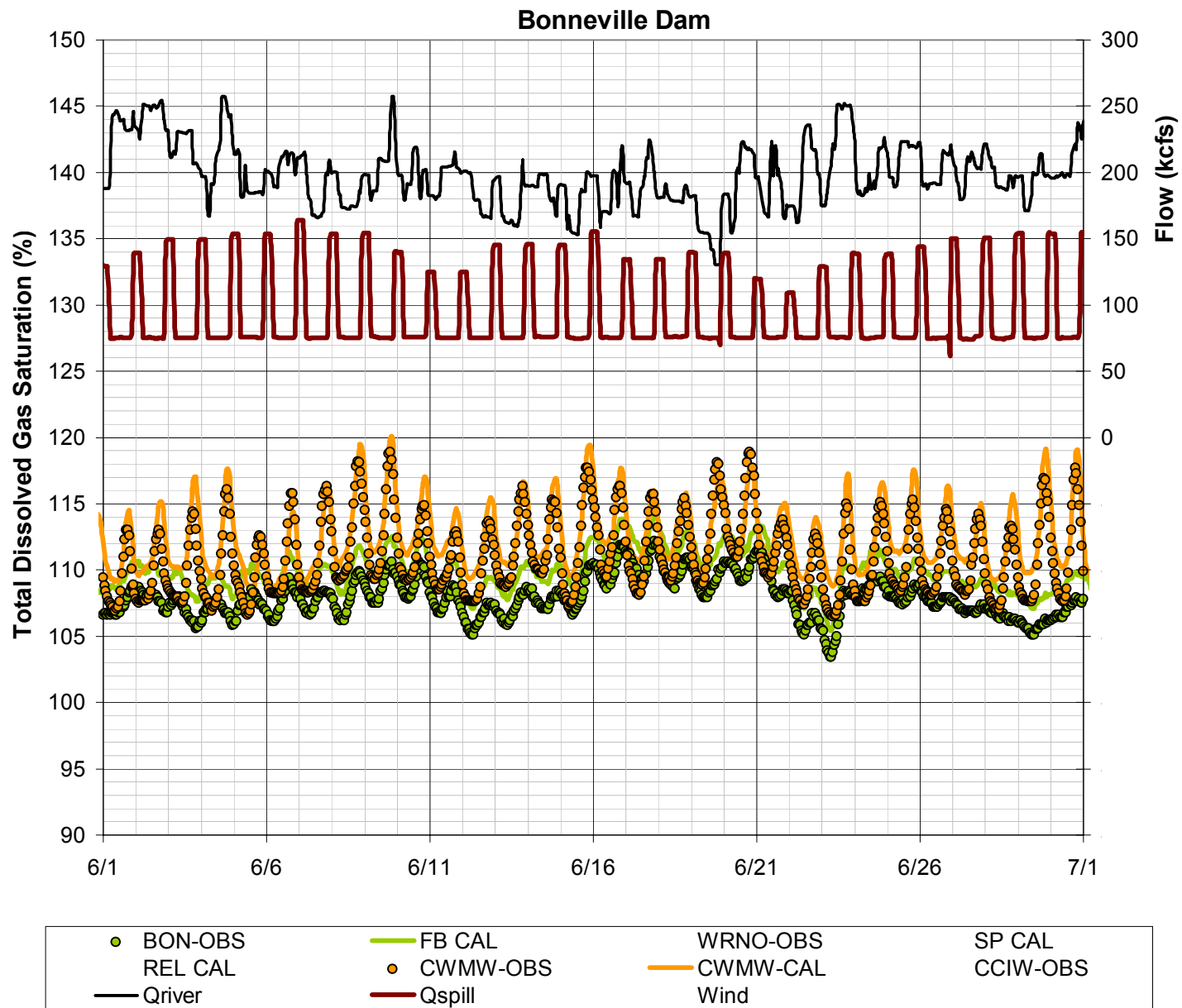
Figure 44. Observed and Calculated TDG Saturation in the Columbia River at Camas/Washougal (CWMW) and in the forebay of Bonneville Dam (BON) during June 2005 (Observed – Base condition, Calculated – spill unchanged from base condition with forebay TDG saturation 2 percent higher than base condition)
