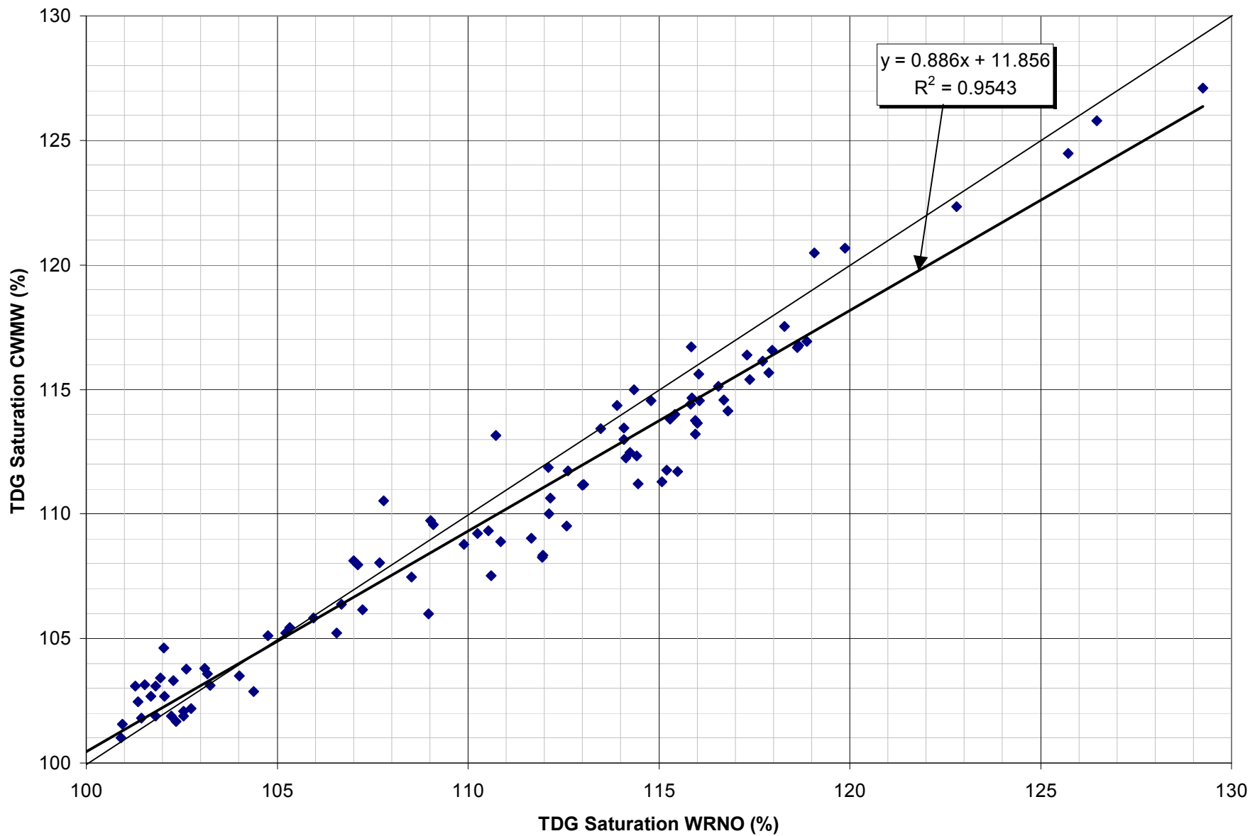
Figure 24. Monthly Average TDG Saturation in the Lower Columbia River at stations CWMW and WRNO, 1994-2005
