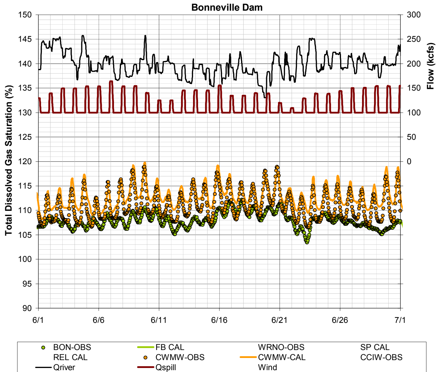
Figure 40. Observed and Calculated TDG Saturation in the Columbia River at Camas/Washougal (CWMW) and in the forebay of Bonneville Dam (BON) during June 2005 (Observed – Base condition; Calculated - daytime spill = 100 kcfs, nighttime spill unaltered from base condition)
