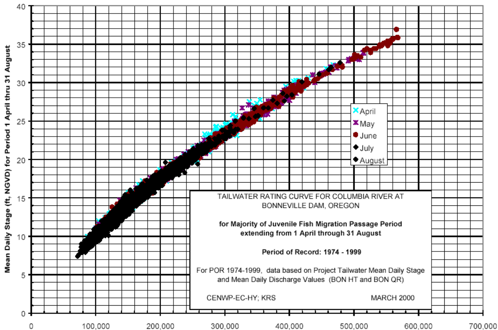
Figure 9. Tailwater Stage Rating Curve for Columbia River at Bonneville Dam 1 April-31 August
