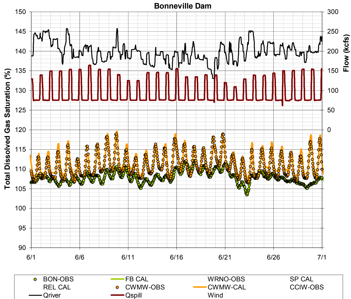
Figure 38. Observed and Calculated TDG Saturation in the Columbia River at Camas/Washougal (CWMW) and in the forebay of Bonneville Dam (BON) during June 2005. (Base Condition – Hourly Historic Flows)
