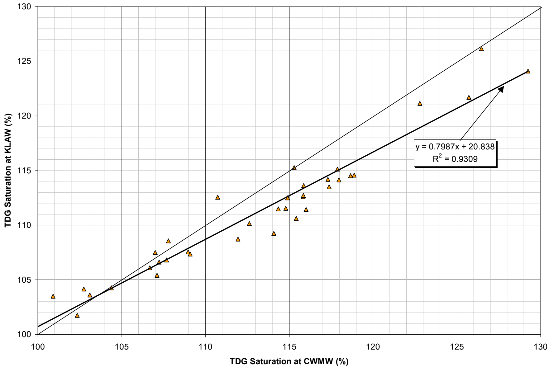
Figure 25. Monthly Average TDG Saturation in the Lower Columbia River at stations CWMW and KLAU, 1994-1998
