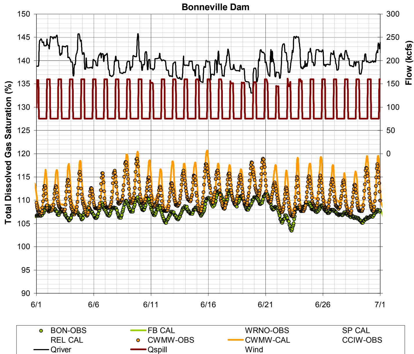
Figure 41. Observed and Calculated TDG Saturation in the Columbia River at Camas/Washougal (CWMW) and in the forebay of Bonneville Dam (BON) during June 2005 (Observed – Base condition; Calculated nighttime spill = 160 kcfs, daytime spill unaltered from base condition)
