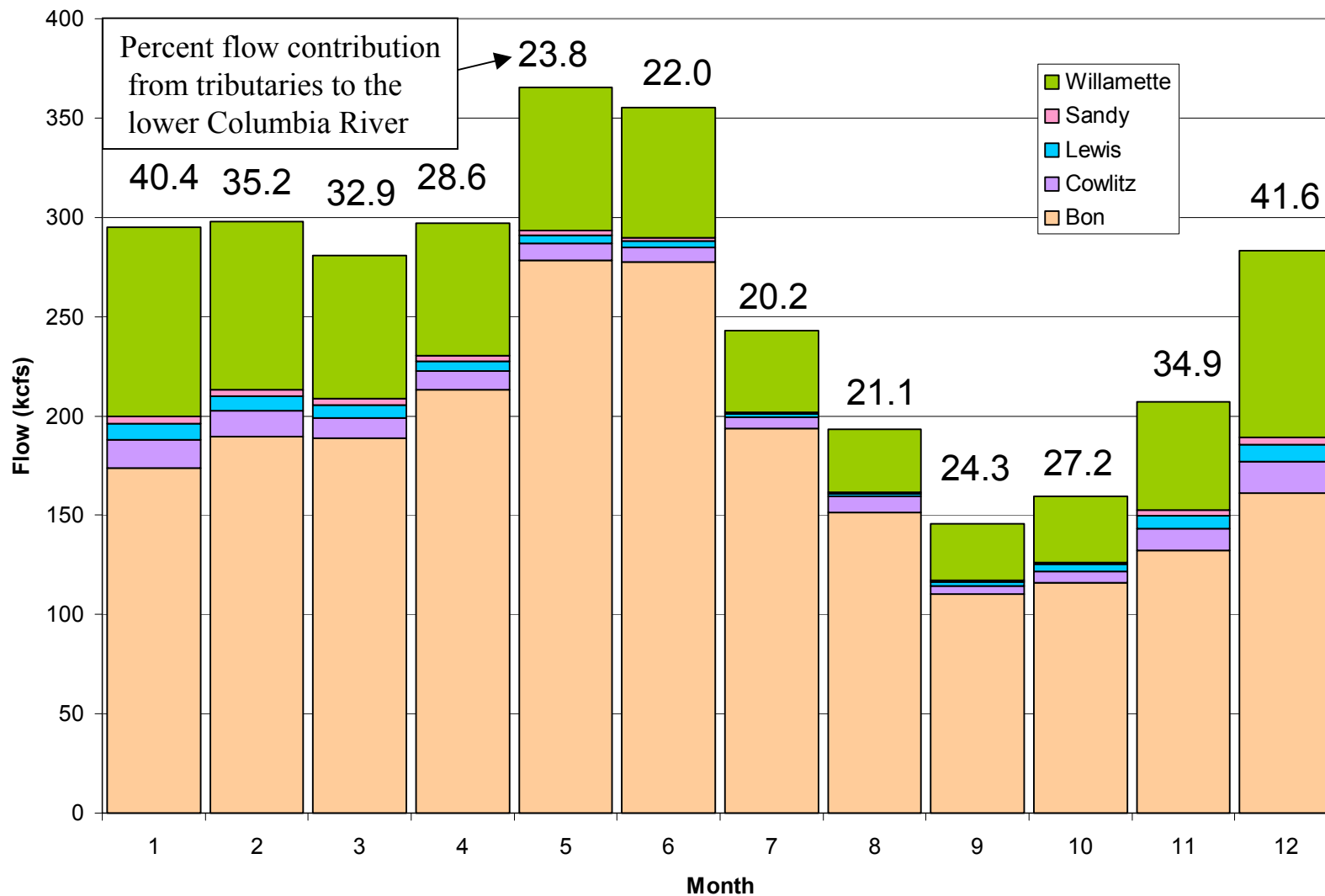
Figure 5. Lower Columbia River Average Monthly Flow Composition, 1993-2005
