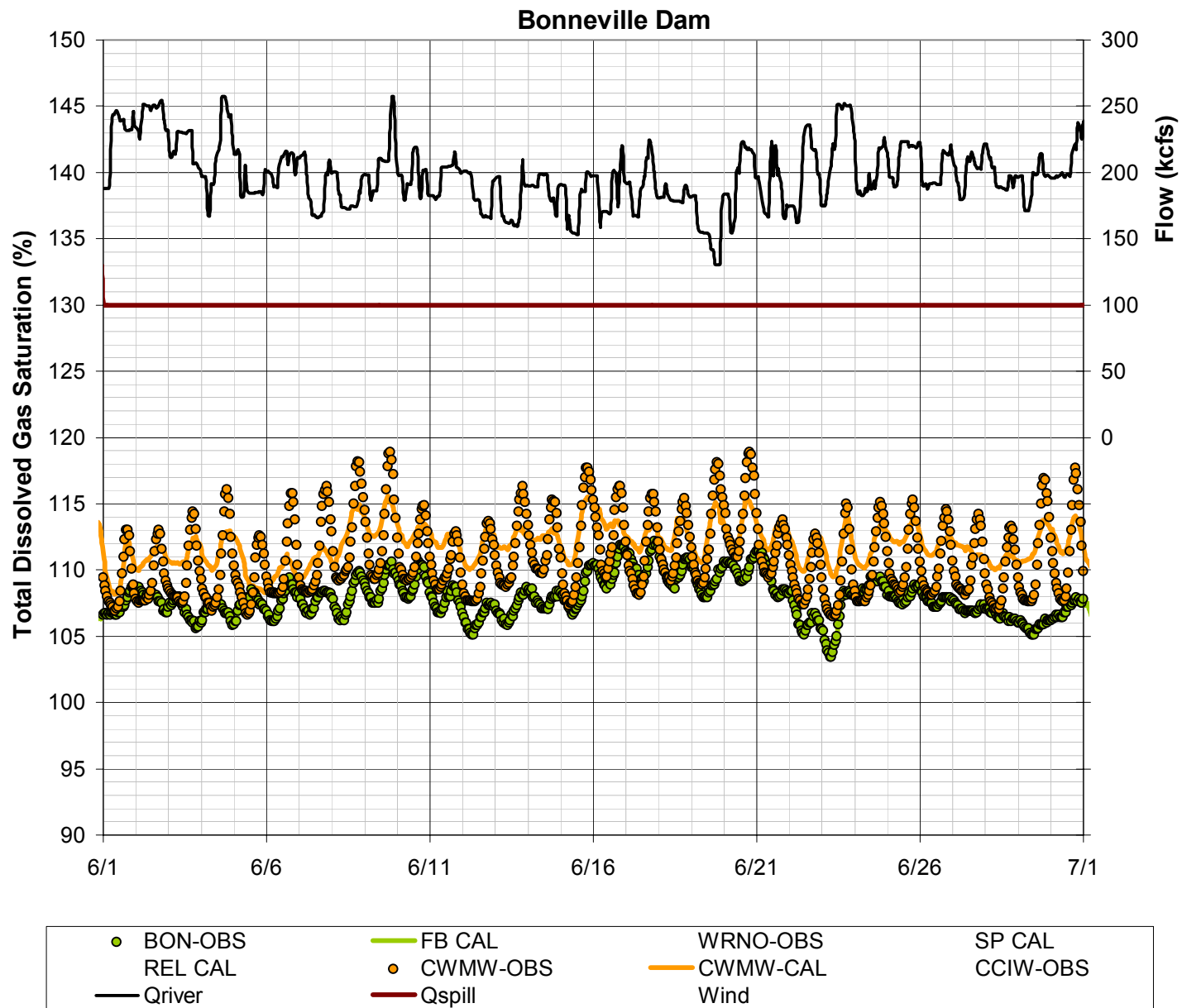
Figure 42. Observed and Calculated TDG Saturation in the Columbia River at Camas/Washougal (CWMW) and in the forebay of Bonneville Dam (BON) during June 2005 (Observed – Base condition, Calculated – continuous 100 kcfs spill)
