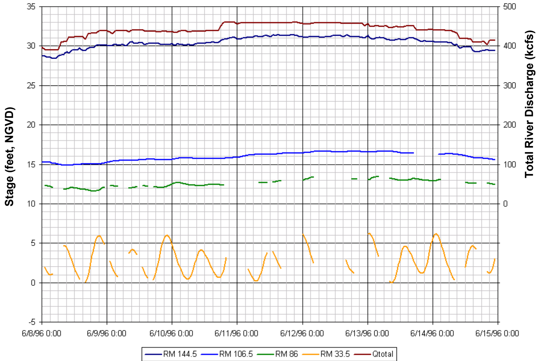
Figure 13. Bonneville Dam Flow and Columbia River Water Surface Elevation for June 8-14, 1996 (Average Bonneville Flow = 441 kcfs)
