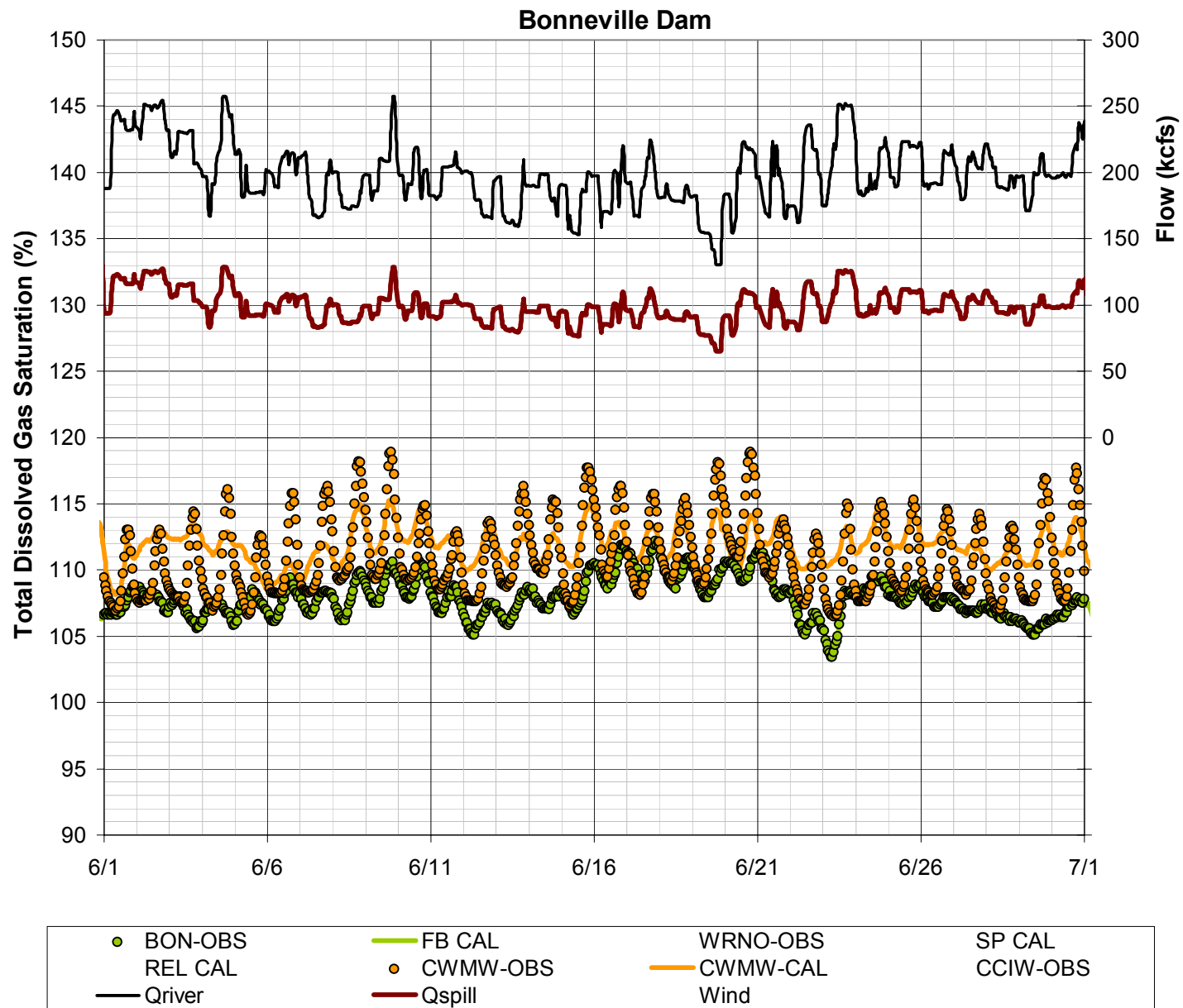
Figure 43. Observed and Calculated TDG Saturation in the Columbia River at Camas/Washougal (CWMW) and in the forebay of Bonneville Dam (BON) during June 2005 (Observed – Base condition, Calculated – spill half of the instantaneous river flow)
