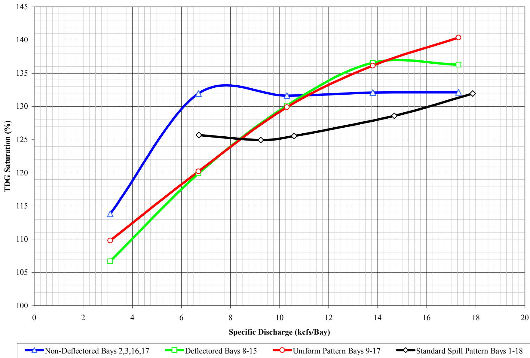
Figure 16. Average Total Dissolved Gas Saturation below Bonneville Spillway as a Function of Spill Pattern and Specific Discharge, February 1-4, 1999.
