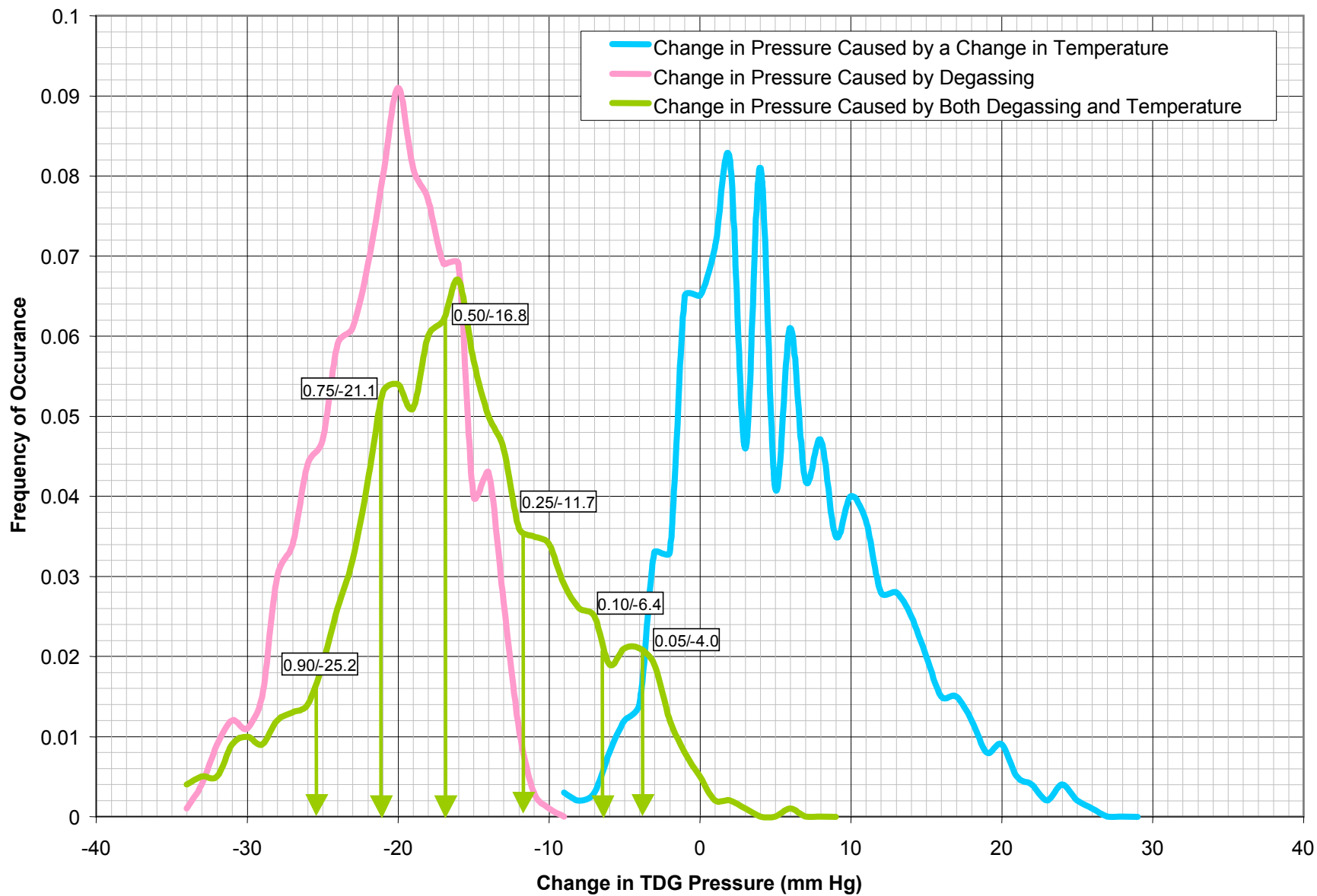
Figure 37. Fate of TDG Pressure in the Columbia River from Bonneville Dam to Camas/Washougal, April-August 2002
