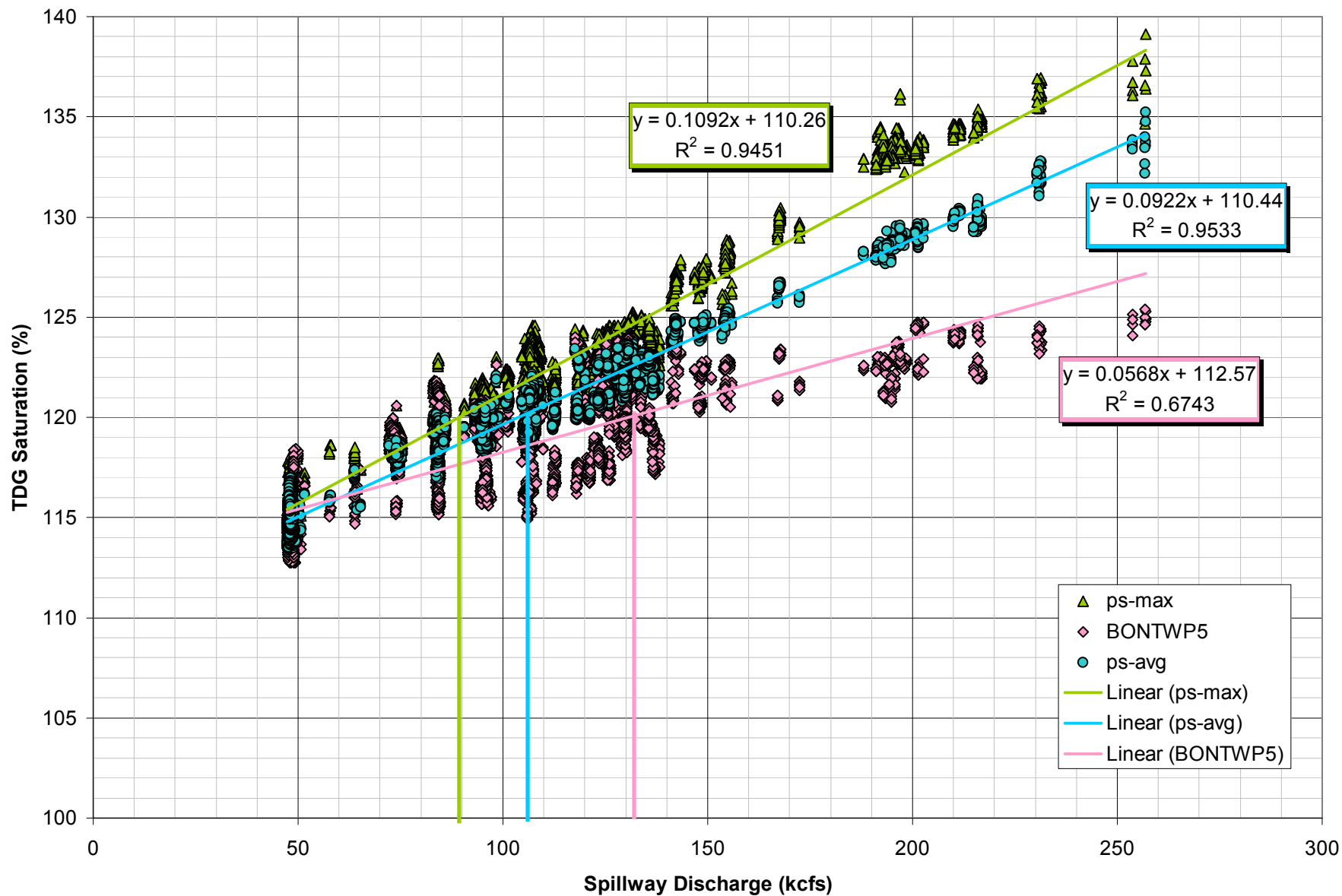
Figure 18. Total Dissolved Gas Saturation in the Bonneville spillway exit channel as a function of spillway discharge, April- July, 2002 (ps-max=maximum cross sectional, ps-avg=average cross sectional, BONTWP5-Cascade Island station)
