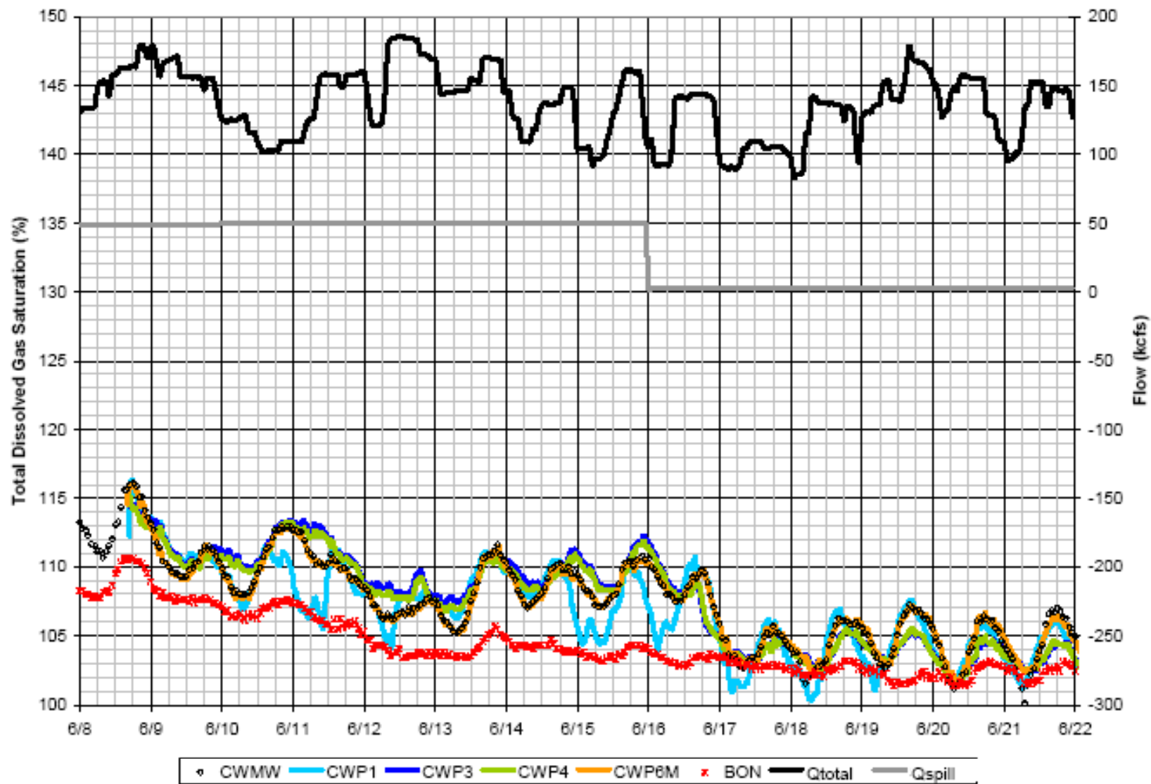
Figure 36. Hourly Columbia River Total Dissolved Gas Saturation at river mile 122, June 2001. (lateral transect CWP1-CWP6 oriented from the Oregon to Washington shore)
