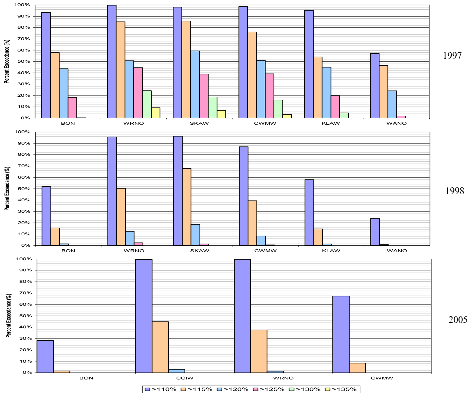
Figure 26. Frequency of Total Dissolved Gas Saturation levels in the Columbia River RM 42-146, 1997, 1998, 2005 (April 15-August 31)
