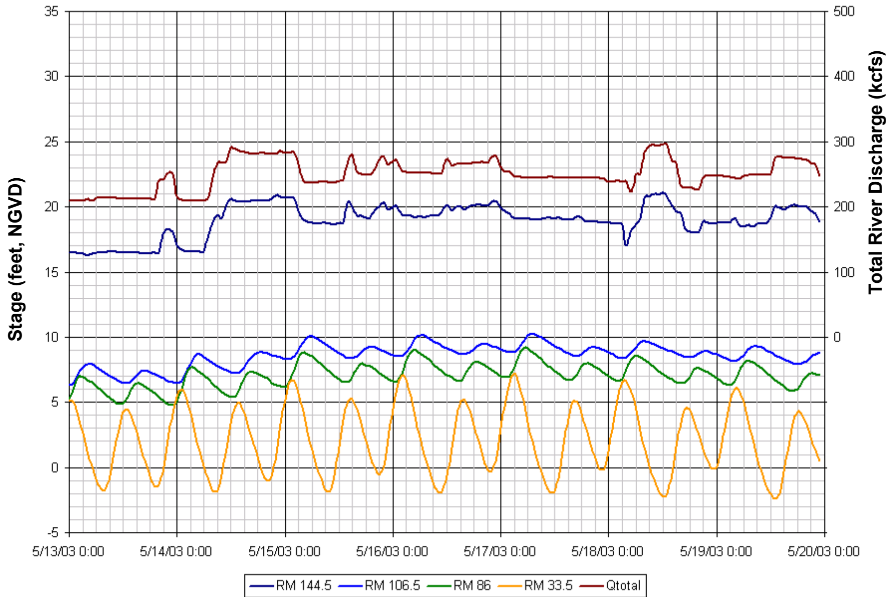
Figure 11. Bonneville Dam Flow and Columbia River Water Surface Elevation for May 13-19, 2003, Average Bonneville Flow = 250 kcfs
