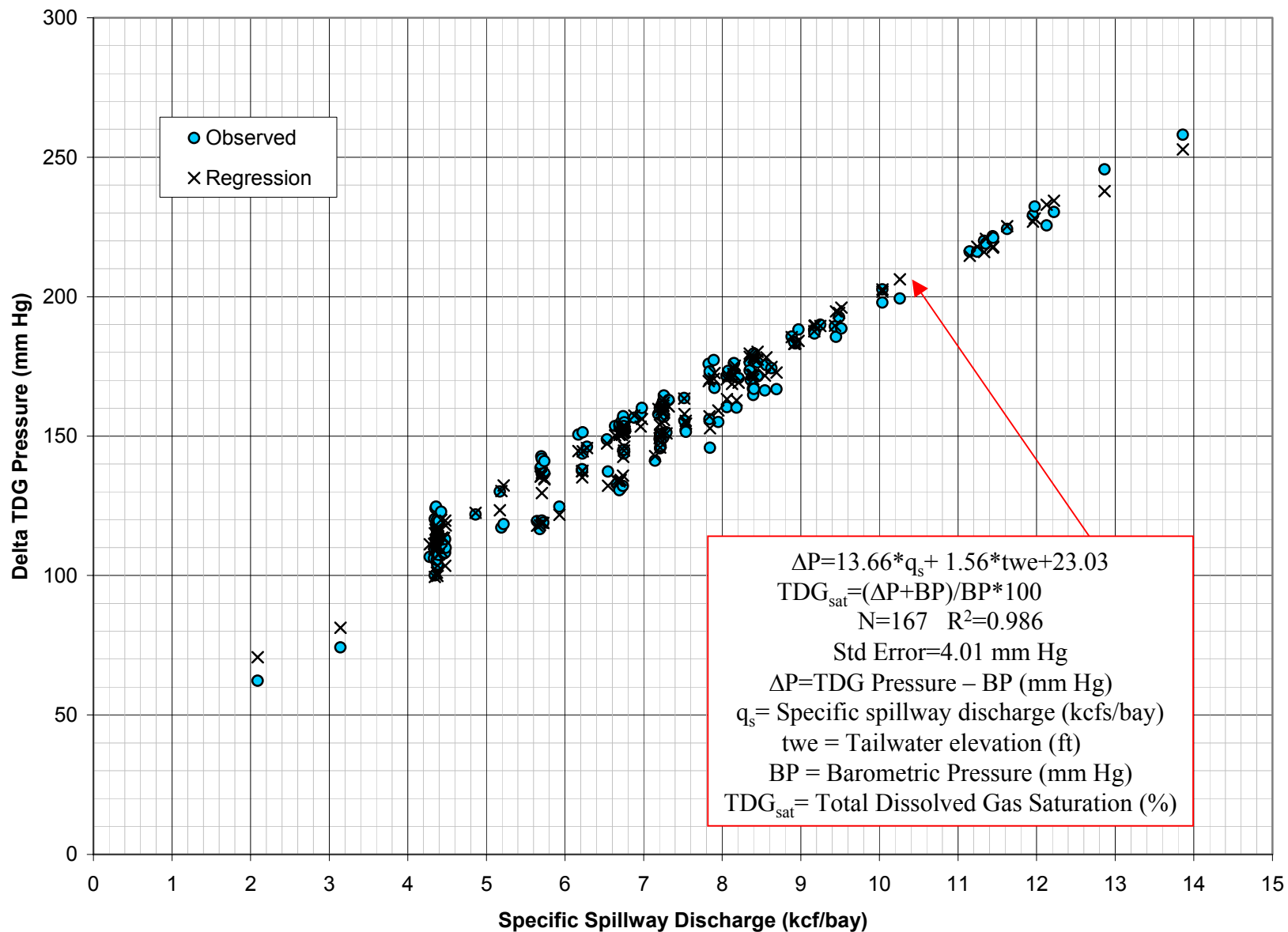
Figure 17. Observed and calculated average cross-sectional delta total dissolved gas pressure in the Bonneville spillway exit channel as a function of tailwater elevation and unit spillway discharge by event
