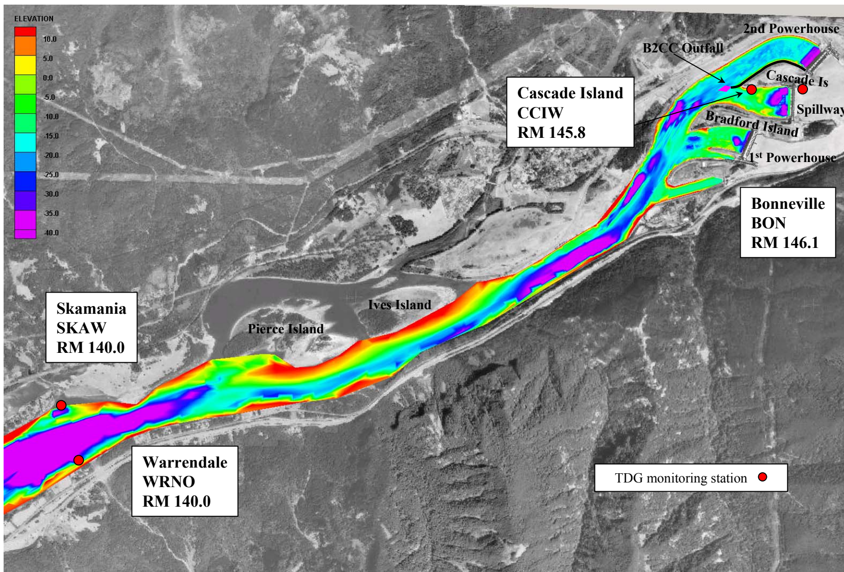
Figure 3. Columbia River Channel Elevations and TDG Fixed Monitoring Stations near Bonneville Dam.
