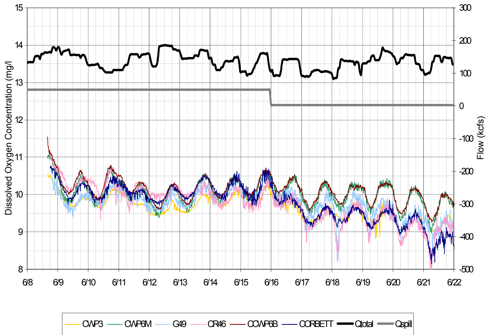
Figure 33. Hourly Columbia River Dissolved Oxygen concentrations at river mile 122, June 2001. (lateral transect CWP1-CWP6 oriented Oregon to Washington shore)
