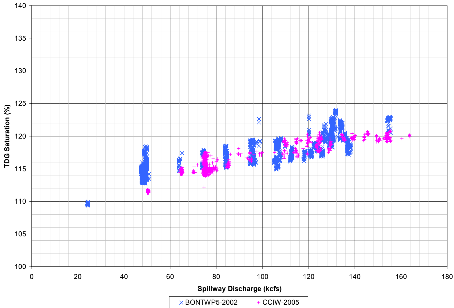
Figure 19. Total Dissolved Gas Saturation as a function of Spillway Discharge at stations BONTWP5 and CCIW.
