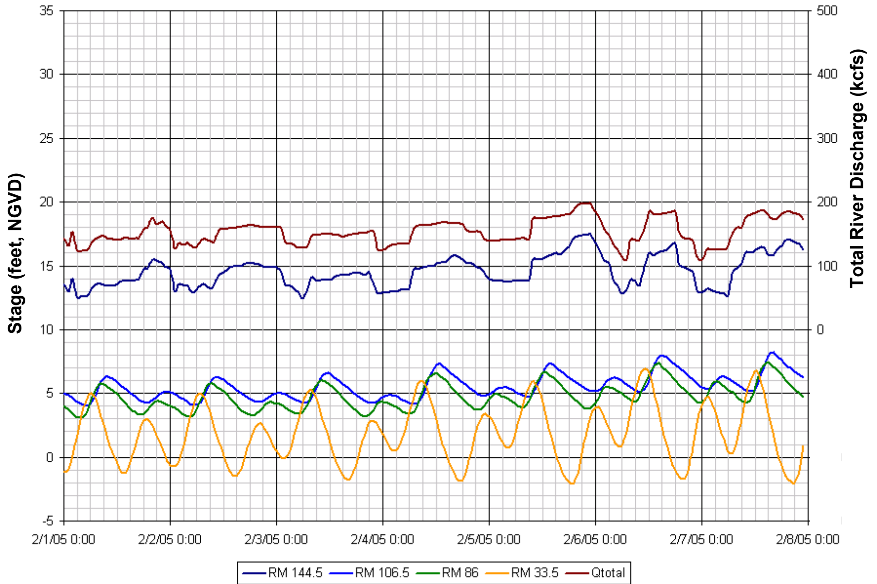
Figure 10. Bonneville Dam Flow and Columbia River Water Surface Elevation for February 1-7, 2005 Average Bonneville Flow = 150 kcfs.
