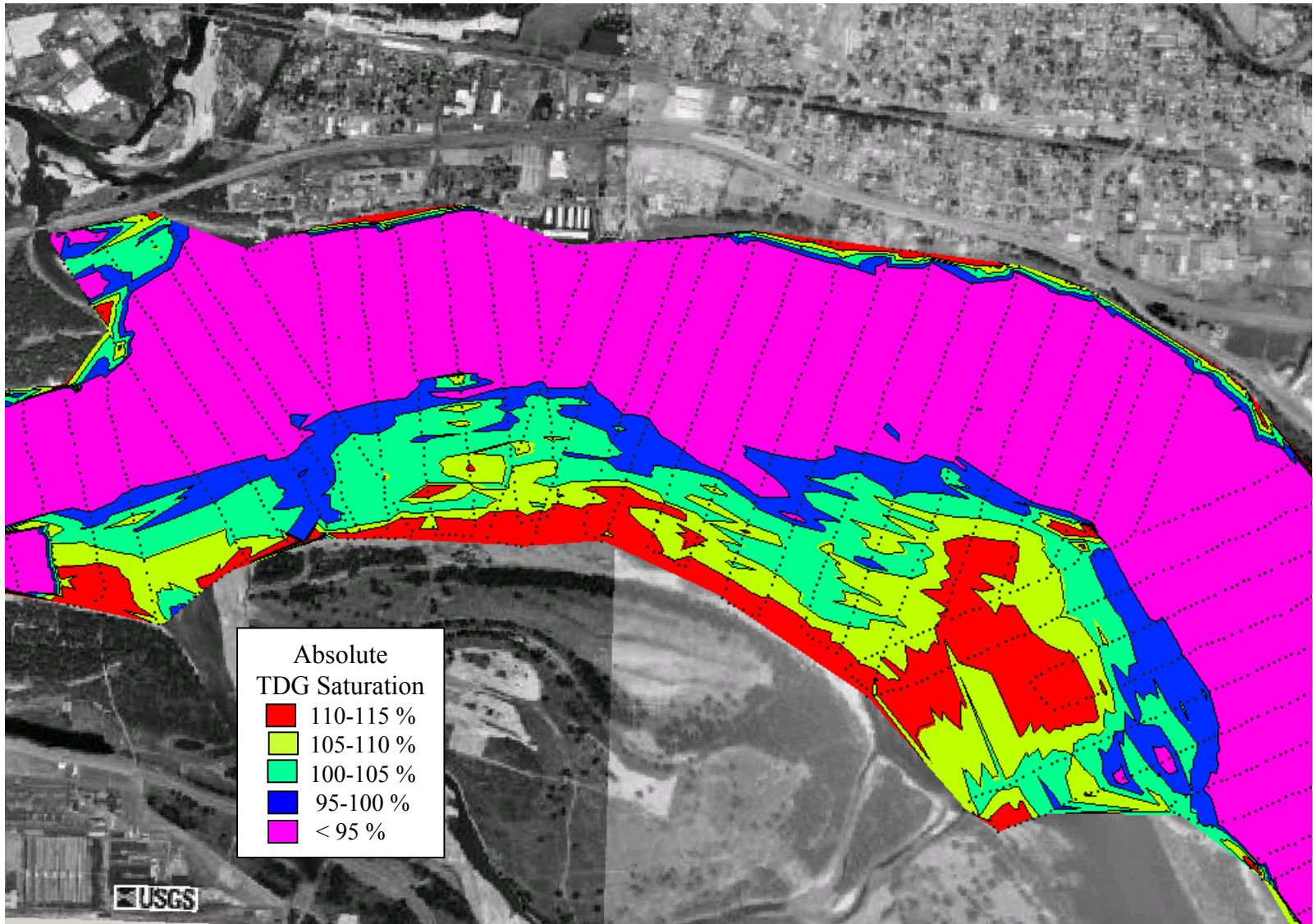
Figure 46. Absolute TDG Saturation at the channel bed of the Columbia River (Stage 10 ft NGVD, TDG Saturation 115%,)
