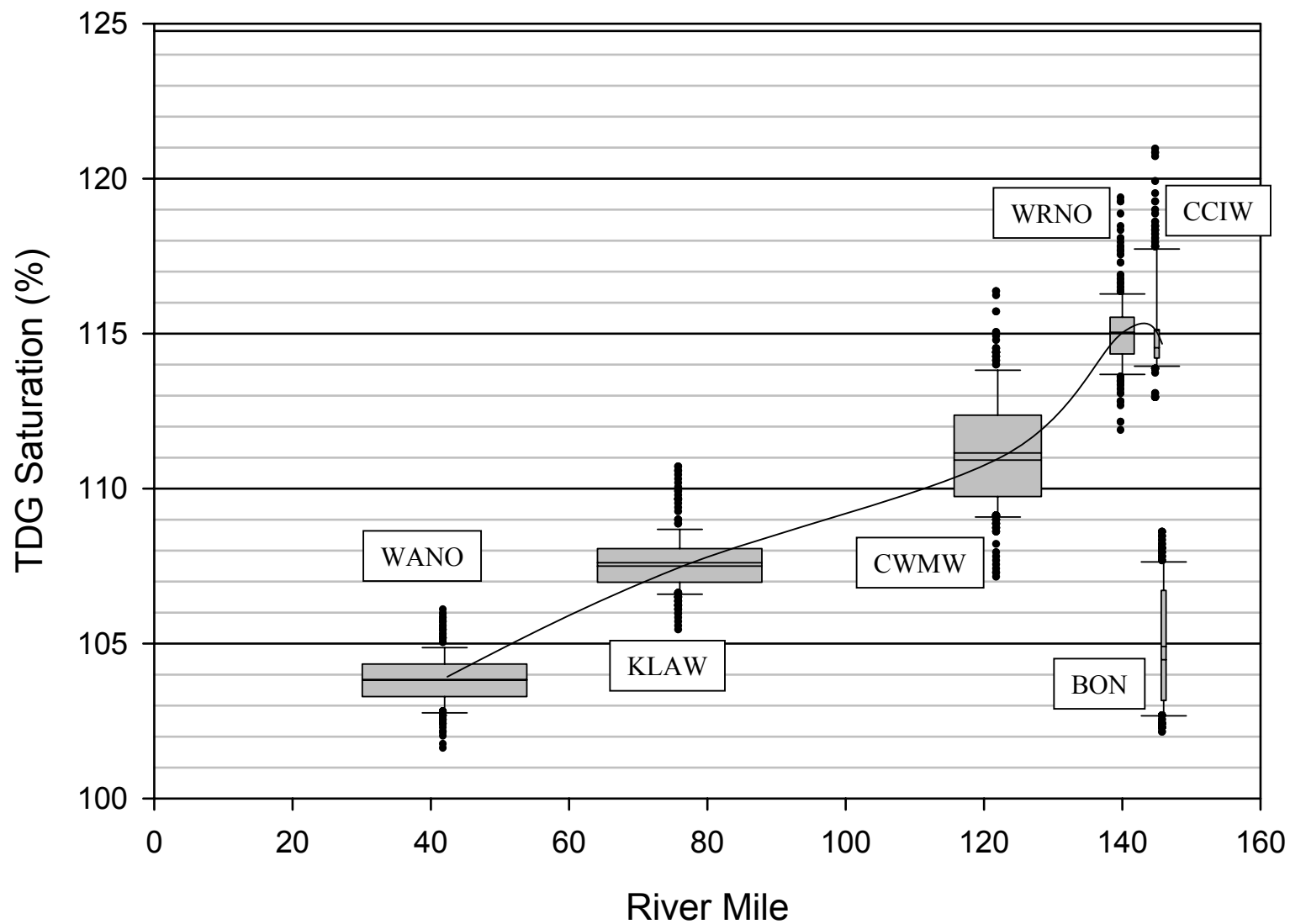
Figure 23. Average of TDG Saturation in the Lower Columbia River, August 12-24, 2005.
