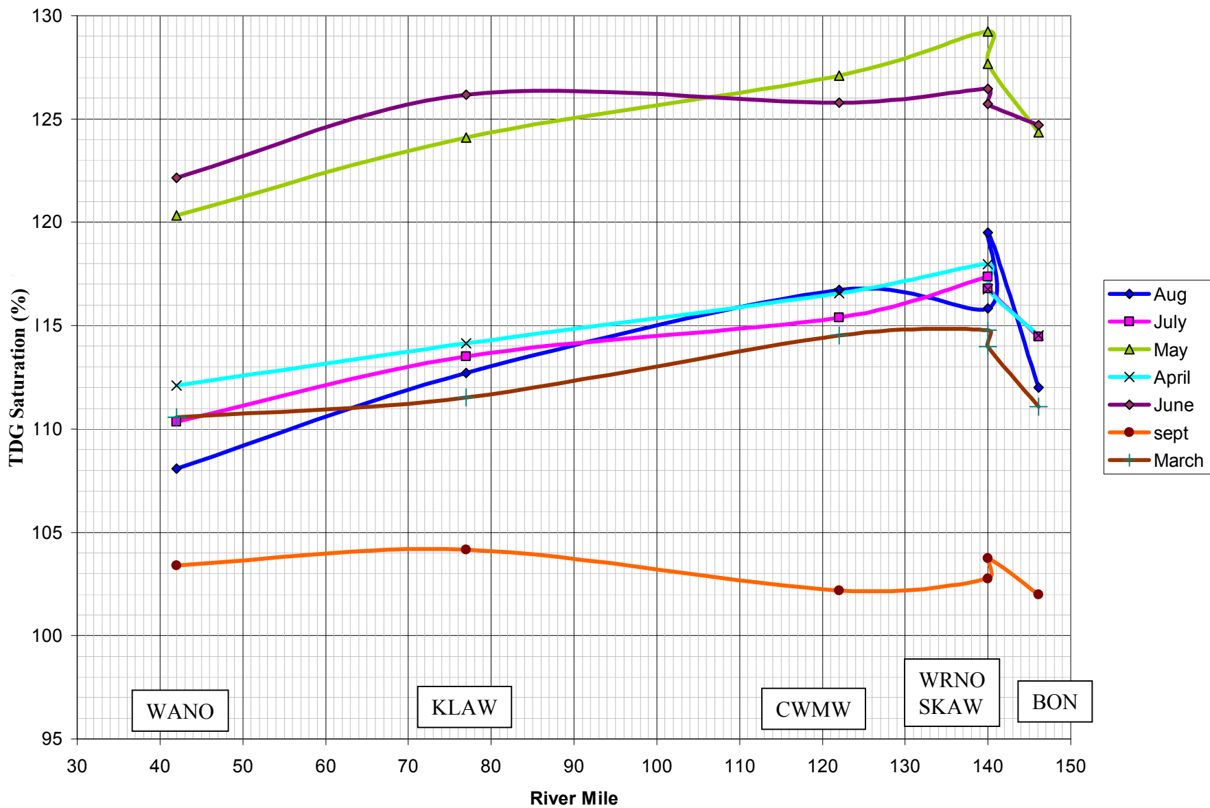
Figure 22. Monthly Average of TDG Saturation for 1997 in the Lower Columbia River.
