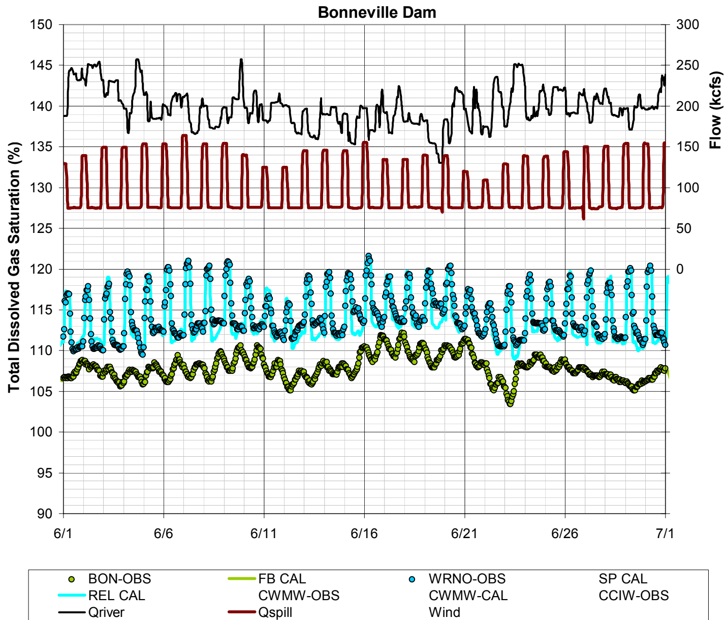
Figure 39. Observed and Calculated TDG Saturation in the Columbia River at Warrendale (WRNO) and in the forebay of Bonneville Dam (BON) during June 2005. (Base Condition – Hourly Historic Flows)
