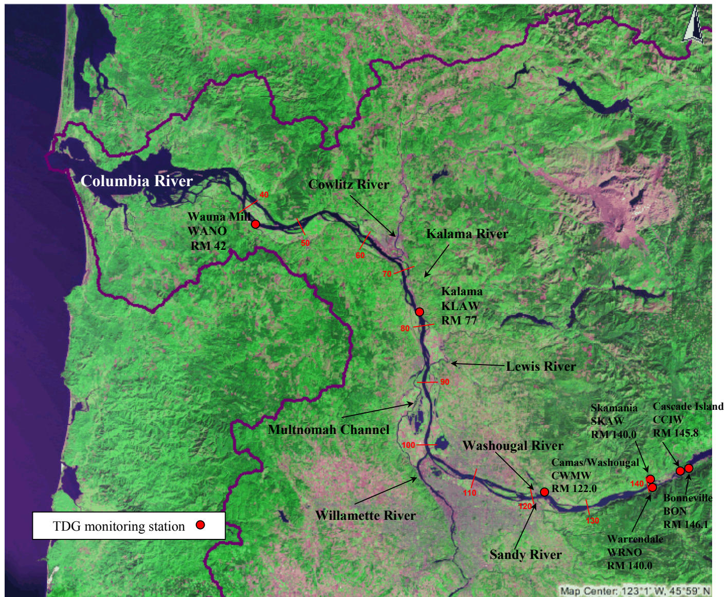
Figure 2. Lower Columbia River and TDG fixed monitoring stations.
