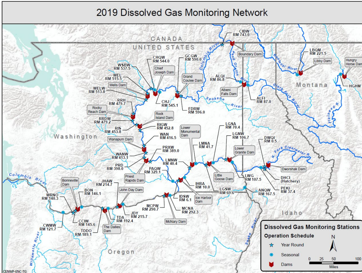
Figure 1 2019 Total Dissolved Gas Fixed Monitoring Stations System
