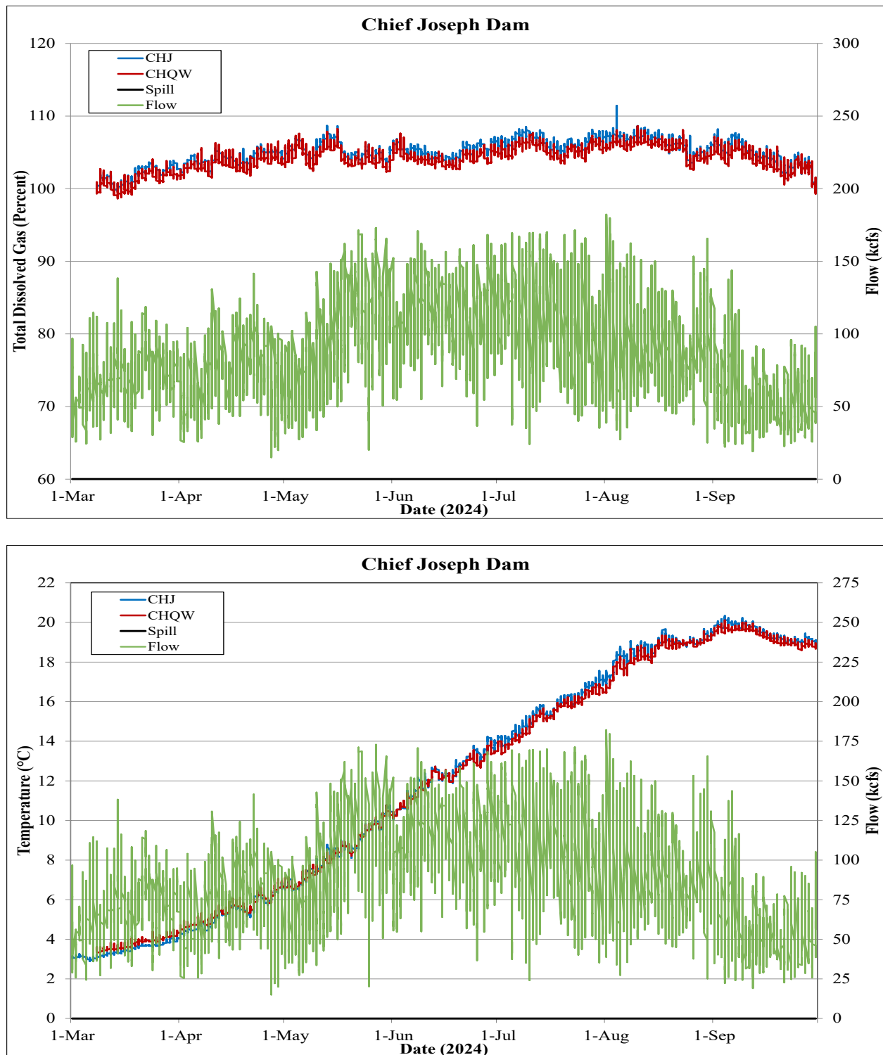
Figure H-6. Percent TDG, spill, and flow (upper panel) and temperature, spill, and flow (lower panel) at Chief Joseph Dam Forebay (CHJ) and Chief Joseph Dam Tailwater (CHQW) stations during spill season 2024.
