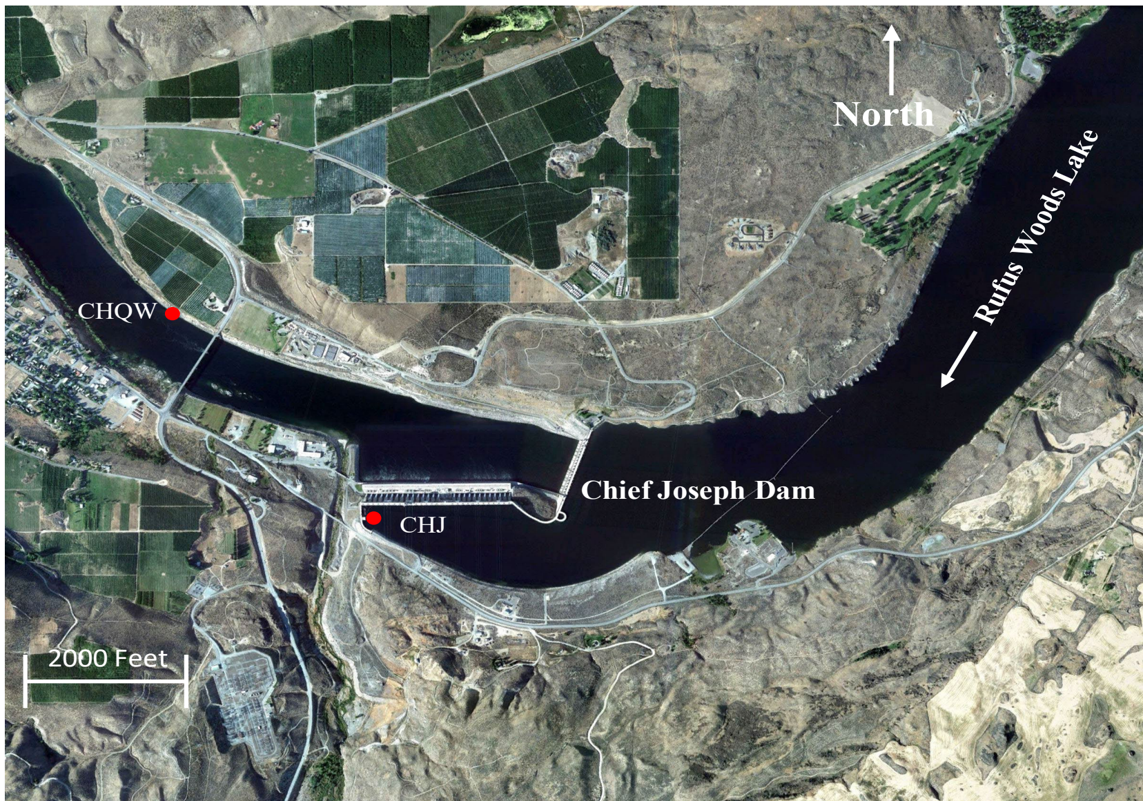
Figure H-3. Locations of TDG monitoring stations in 2024 for Chief Joseph Dam, Washington.
