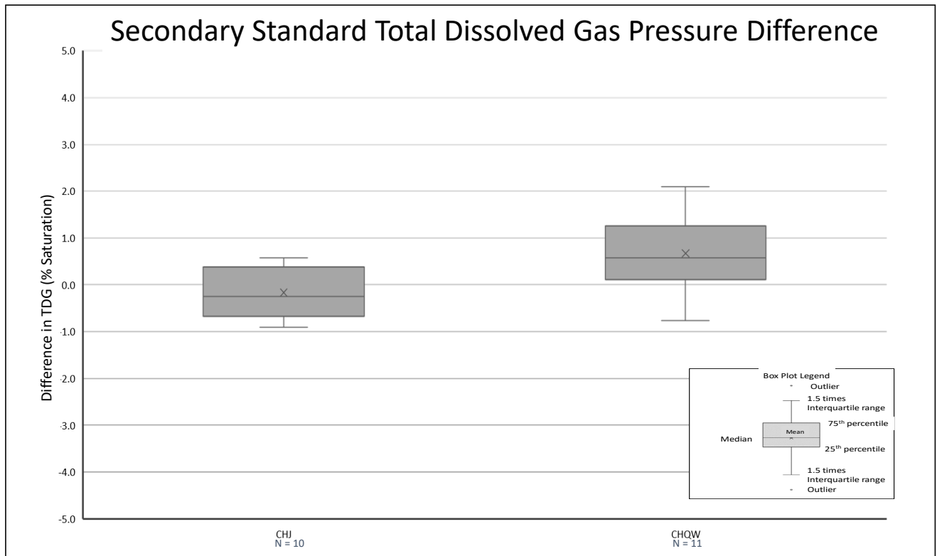
Figure E-5. Difference between the secondary standard and the field TDG instrument for TDG pressure during spill season 2021.
