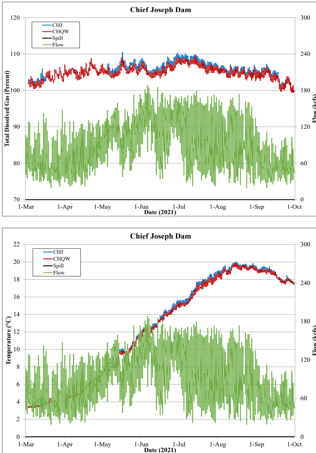
Figure E-6. Percent TDG, spill, and flow (upper panel) and temperature, spill, and flow (lower panel) at Chief Joseph Dam Forebay (CHJ) and Chief Joseph Dam Tailwater (CHQW) stations during spill season 2021.
